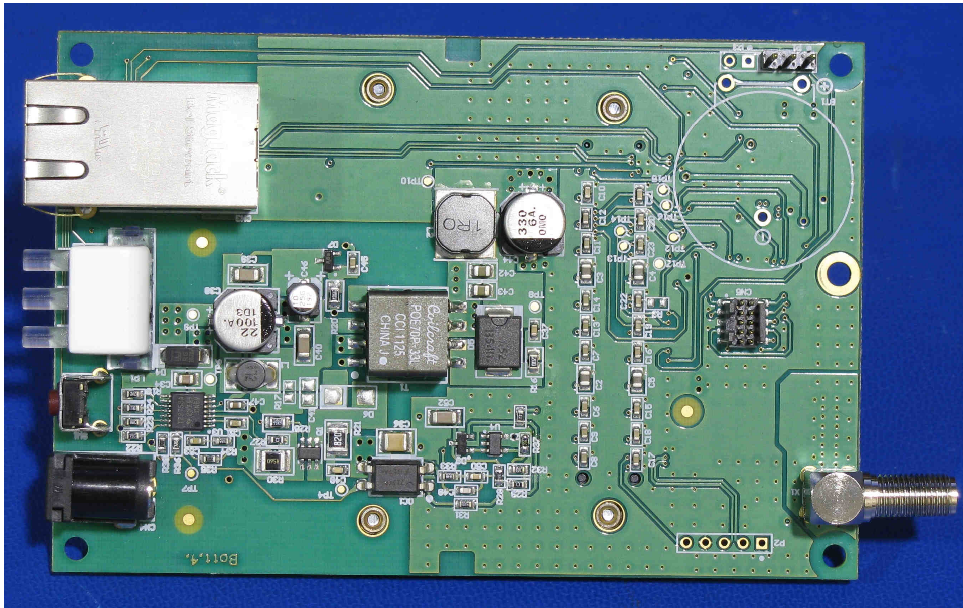
Mother Card, Top Side
