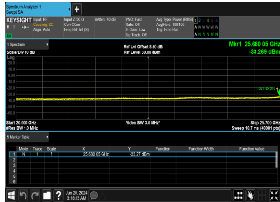
B2_N7(40M)_DFT-s- OFDM_BPSK_Edge_1RB_Left_Mid_CH
