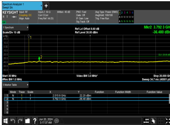
B2_N7(40M)_DFT-s- OFDM_BPSK_Edge_1RB_Left_Mid_CH
