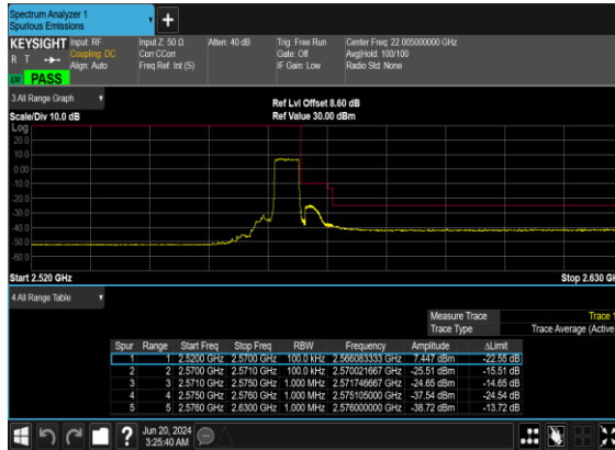
B2_N7(5M)_DFT-s- OFDM_BPSK_Outer_Full_High_CH
