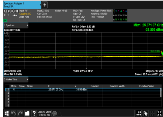
B2_N7(40M)_DFT-s- OFDM_QPSK_Edge_1RB_Left_Mid_CH
