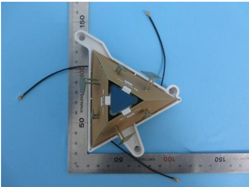
(2) EUT Photo (Panel Antenna, Gain = 4.0dBi)
