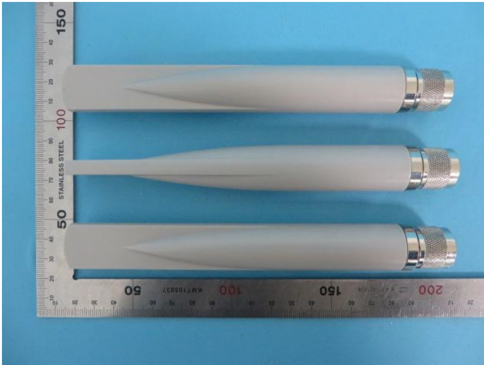
(1) EUT Photo (Panel Antenna, Gain = 4.5dBi)
