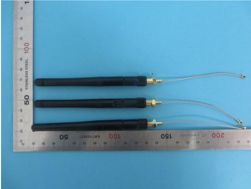
(3) EUT Photo (Dipole Antenna, Gain = 2.0dBi)
