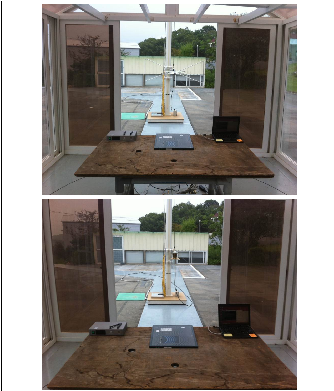
Figure.1. Radiated Emission Test Setup
