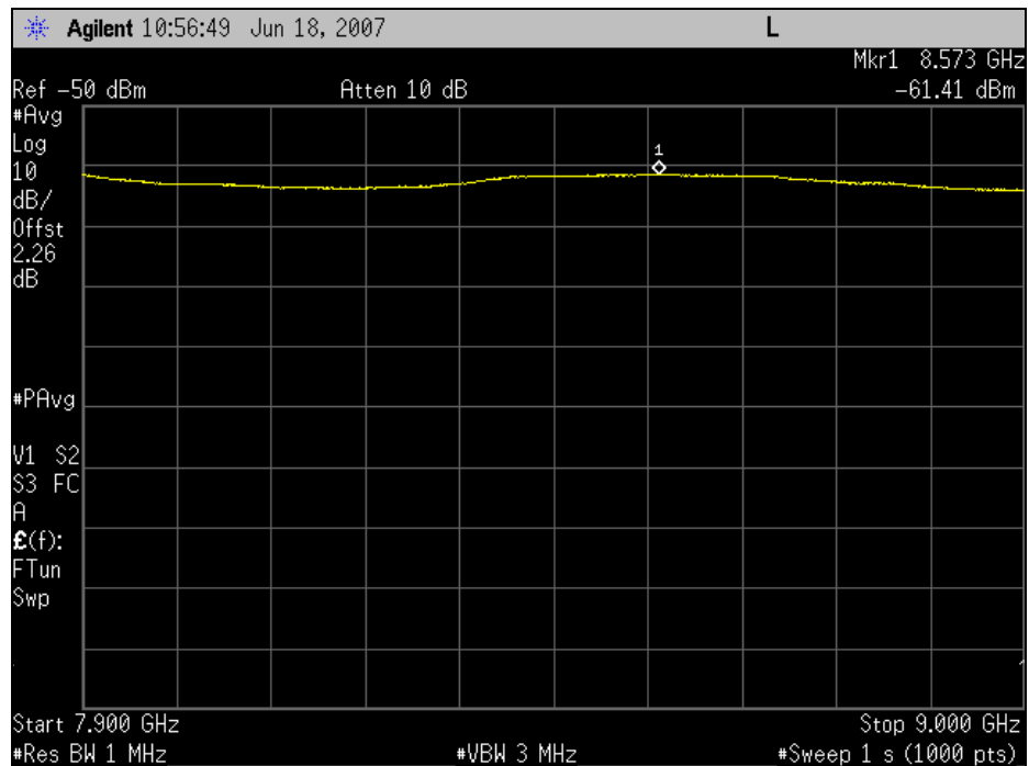
Figure 17. 7.9-9.0 GHz EIRP, Measured @ 1m, Corrected Plot
