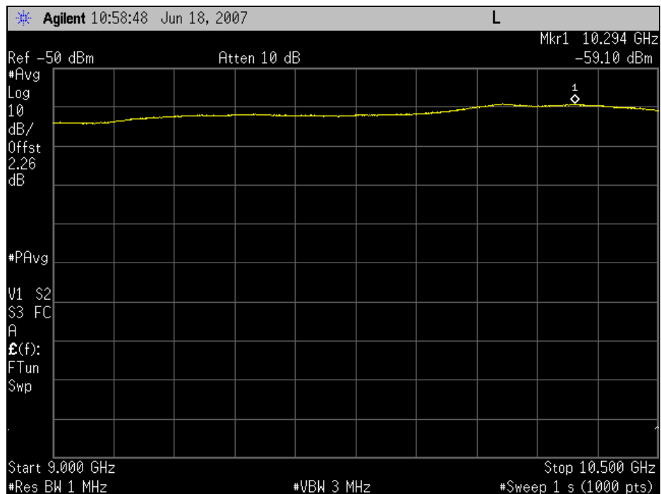
Figure 18. 9.0-10.5 GHz EIRP, Measured @ 1m, Corrected Plot
