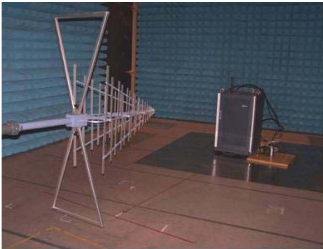
Radiated Emissions- Front View (Below 1 GHz)
