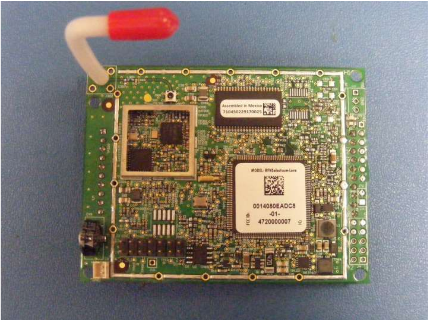
Figure 3: RFN SelectComm 1272 (12V) – Top, shield removed
