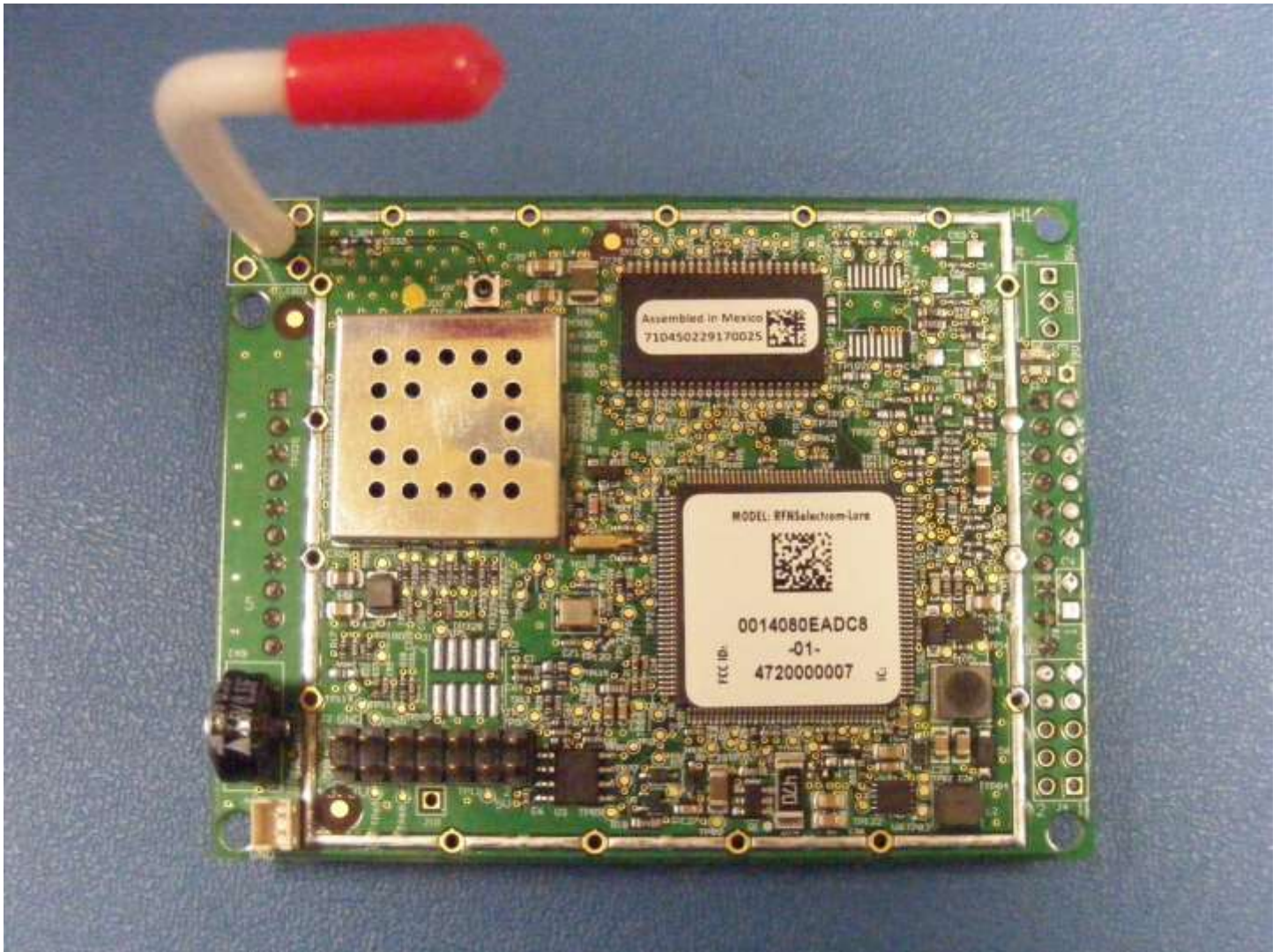
Figure 1: RFN SelectComm 1272 (12V) - Top
