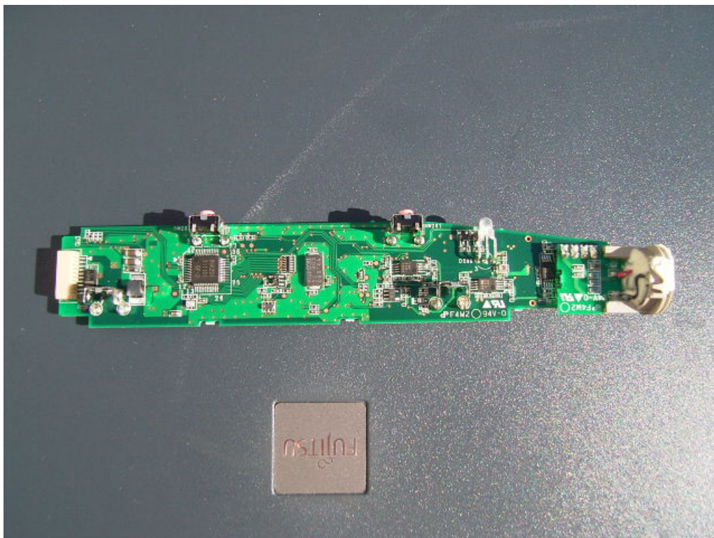
Main board side A (with Antenna board)
