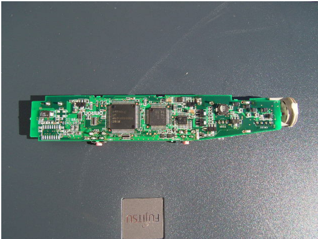
Main board side B (without shield)
