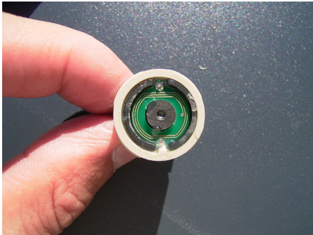
Antenna coil (without Silicone)
