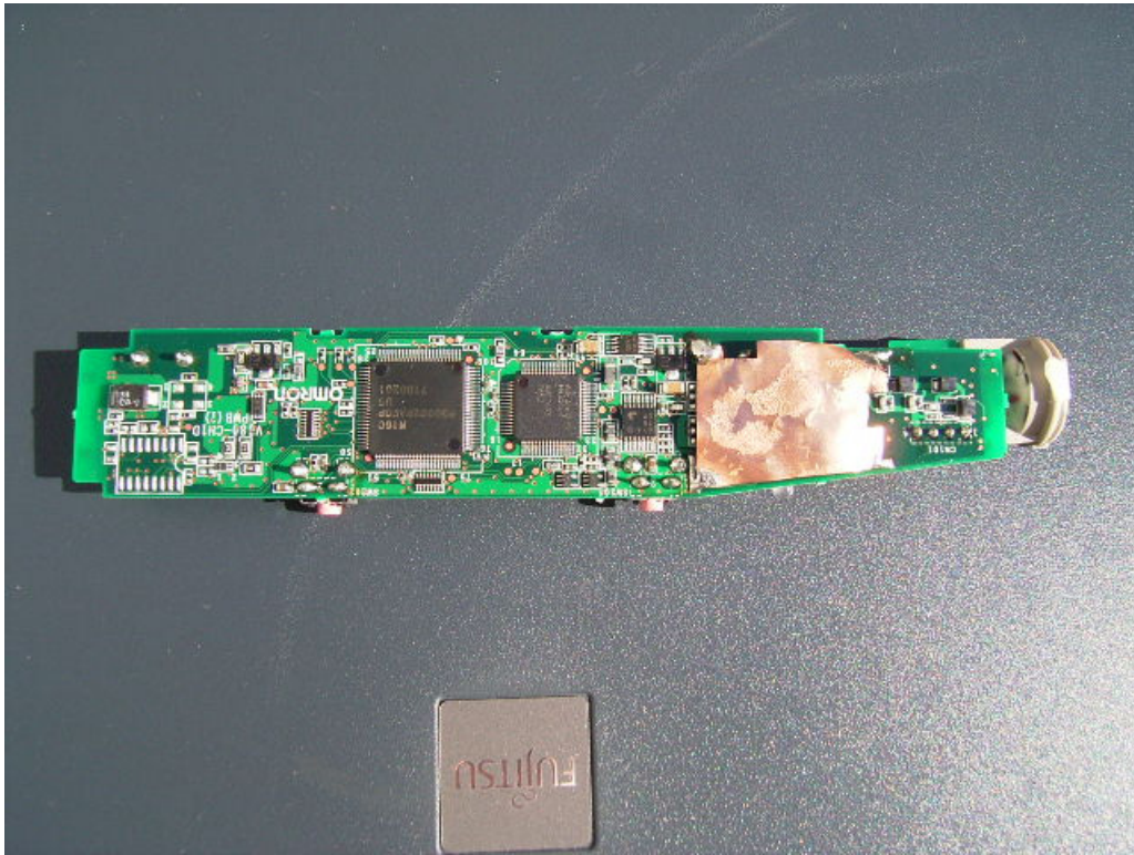
Main board side B (with shield)
