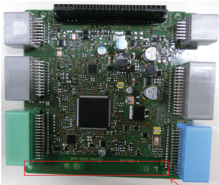
Figure 8.1 K73R0 PCB assy (top view)
