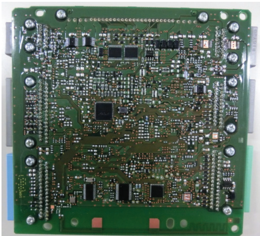
Figure 8.2 K73R0 PCB assy (bottom view)
