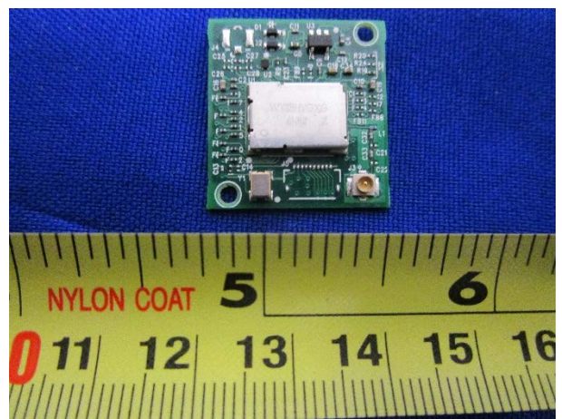
WLAN Radio Module - Bottom View
