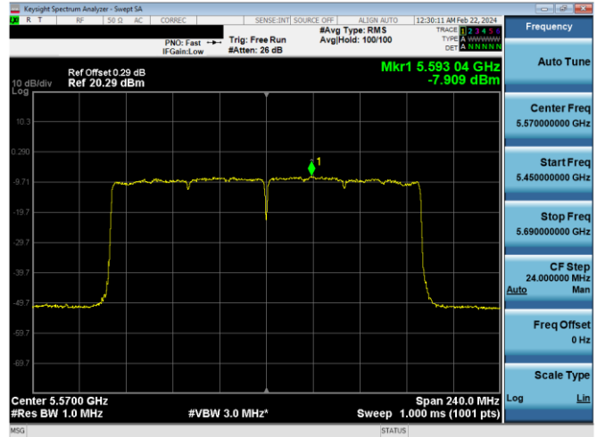
Plot 7-664. PSD CDD Primary Antenna 4a (160MHz BW 802.11ax(SU) – Ch. 114, MCS4)
