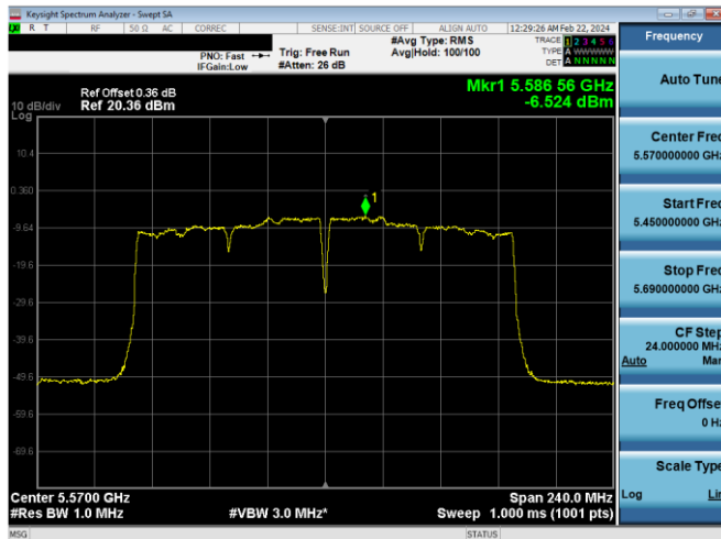
Plot 7-662. PSD CDD Primary Antenna 4a (160MHz BW 802.11ac – Ch. 114, MCS4)
