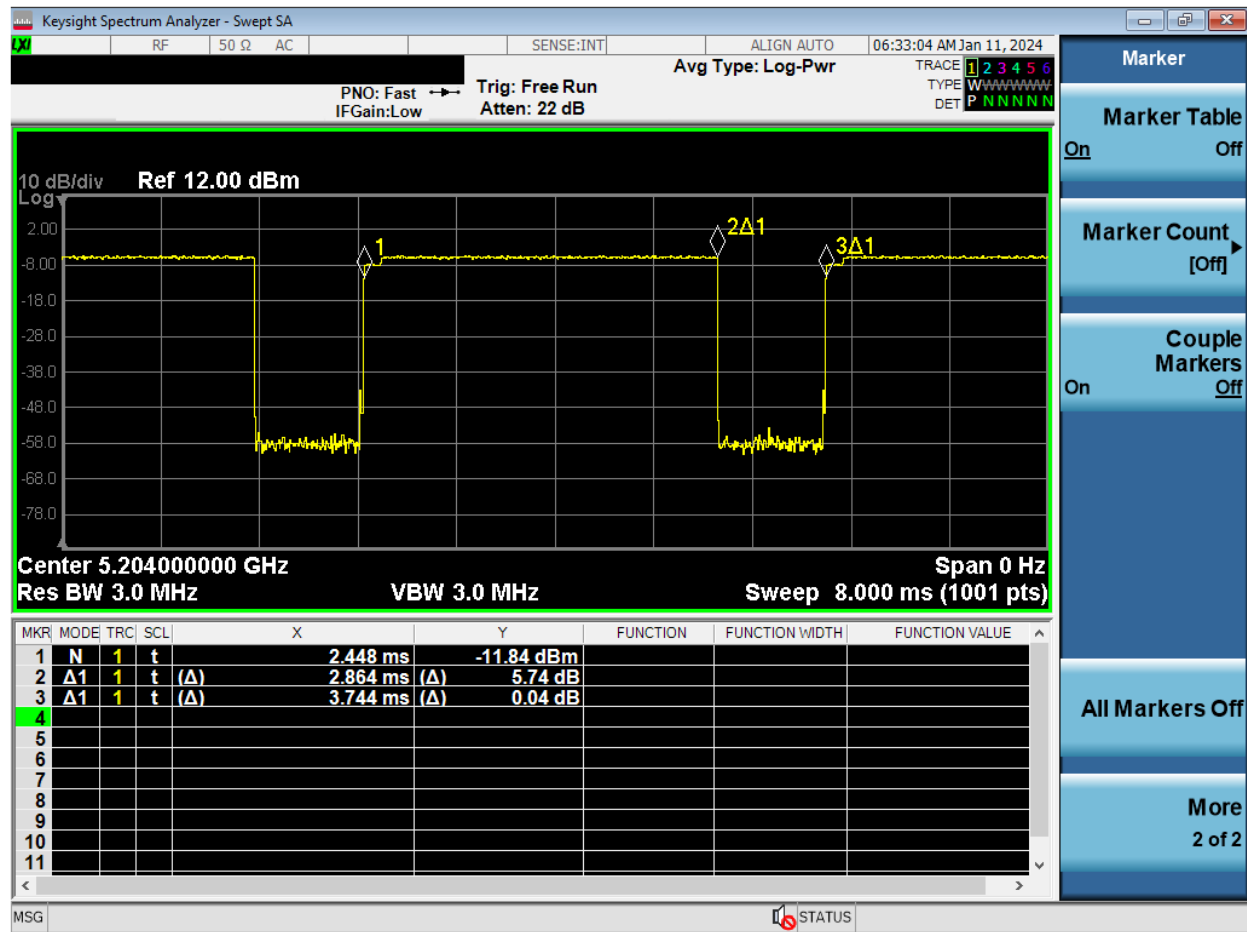
Figure 8-12 NB UNII-1 HDR4 Transmission Plot – Antenna WF5B, Variant 1
