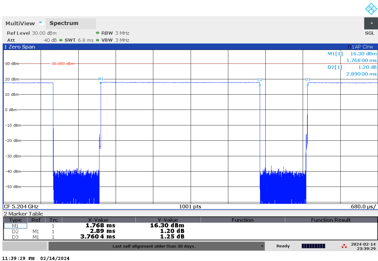
Figure 8-17 NB UNII-1 BDR Transmission Plot – Antenna 2a, Variant 2
