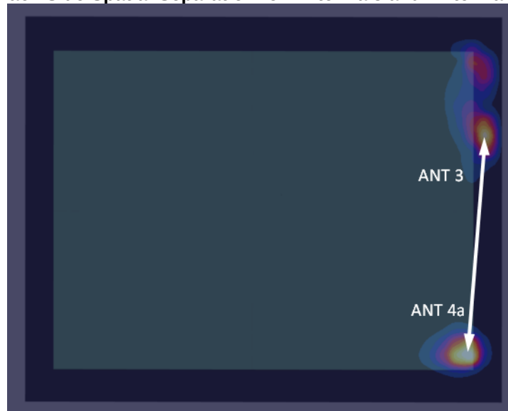
Figure 11-10 Back Side Spatial Separation for Antenna 3 and Antenna 4a
