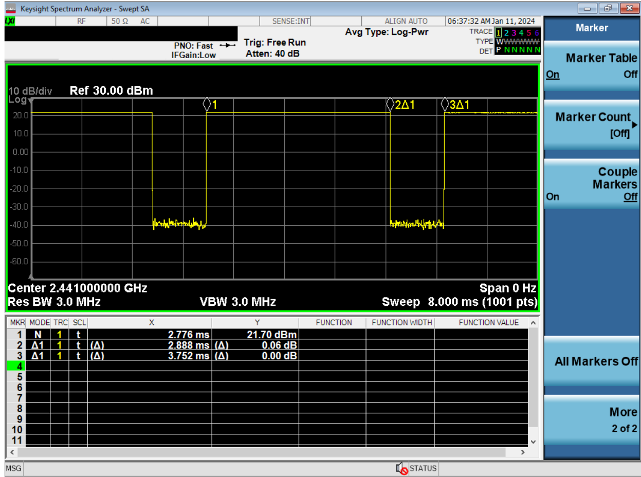
Figure 8-7 Bluetooth Transmission Plot – Antenna 2a, Variant 1
