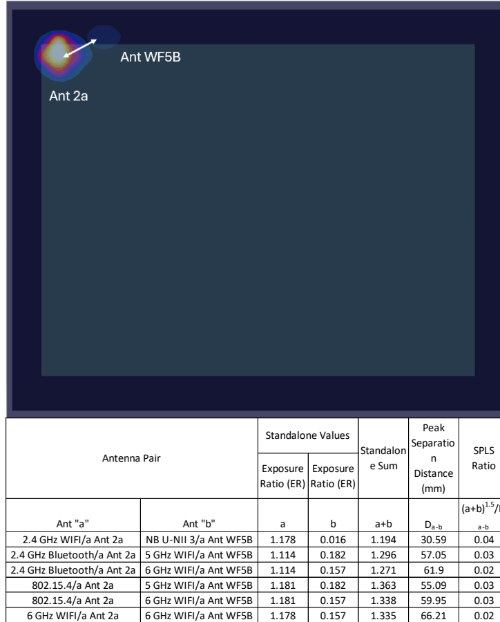
Figure 11-7 Back Side Spatial Separation for Antenna 2a and Antenna WF5B
