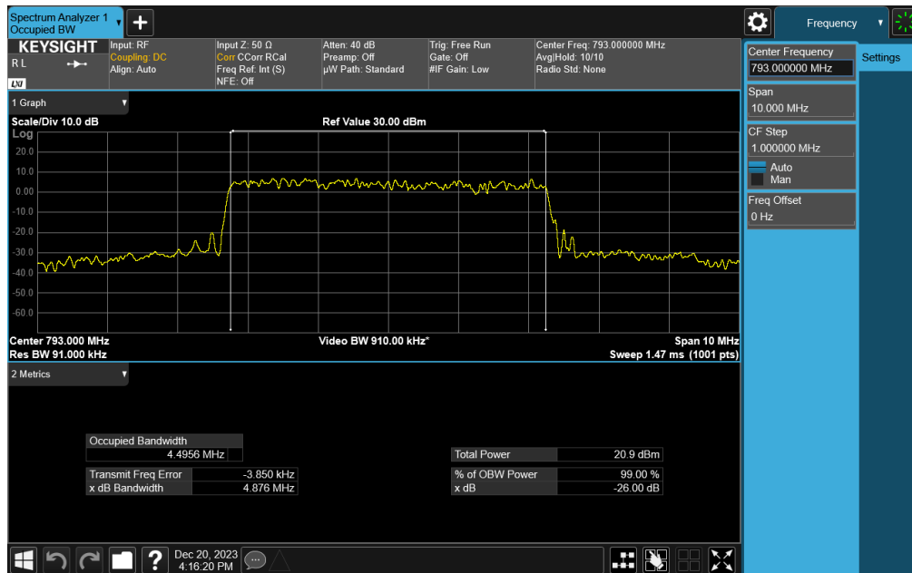
Plot 7-29. Occupied Bandwidth Plot (NR Band 14 - 5MHz DFT-s-OFDM 256-QAM - Full RB)
