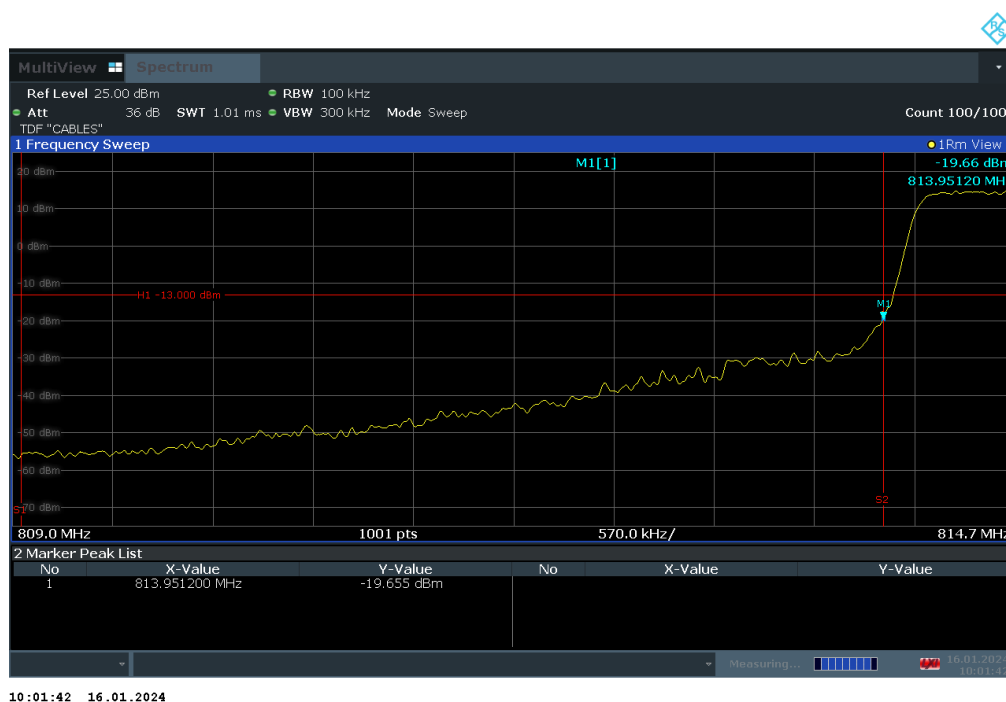
Plot 7-90. Channel Edge Plot (LTE Band 26 – 1.4MHz QPSK – Low Channel)
