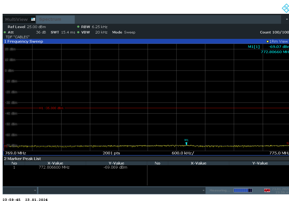
Plot 7-99. Lower Emission Mask Plot (LTE Band 14 - 5MHz QPSK – RB Size 25)
