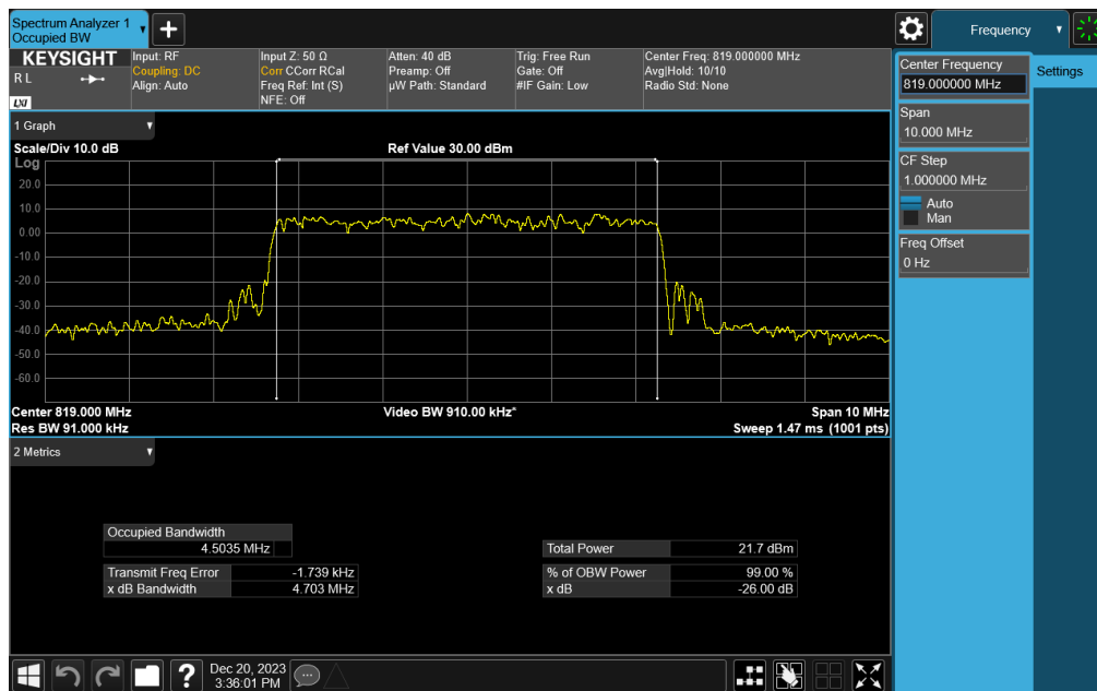
Plot 7-38. Occupied Bandwidth Plot (NR Band 26 - 5MHz CP-OFDM 64-QAM - Full RB)
