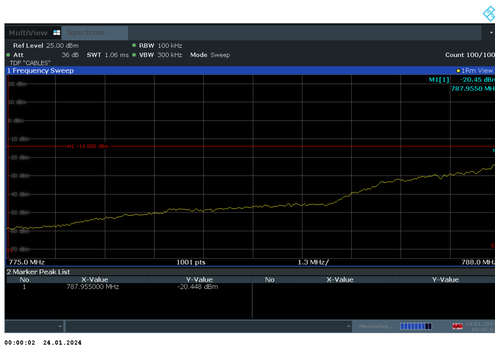
Plot 7-98. Lower Band Edge Plot (LTE Band 14 - 5MHz QPSK – RB Size 25)
