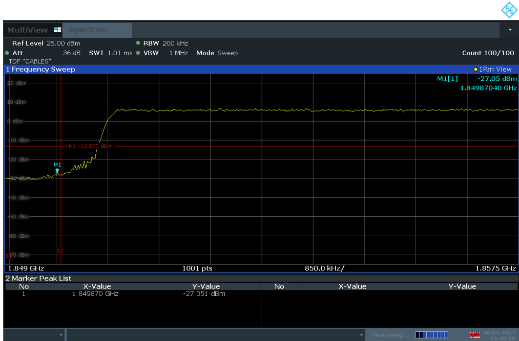
Plot 7-109. Lower Band Edge Plot (LTE Band 25 – 15MHz QPSK – Full RB Configuration)
