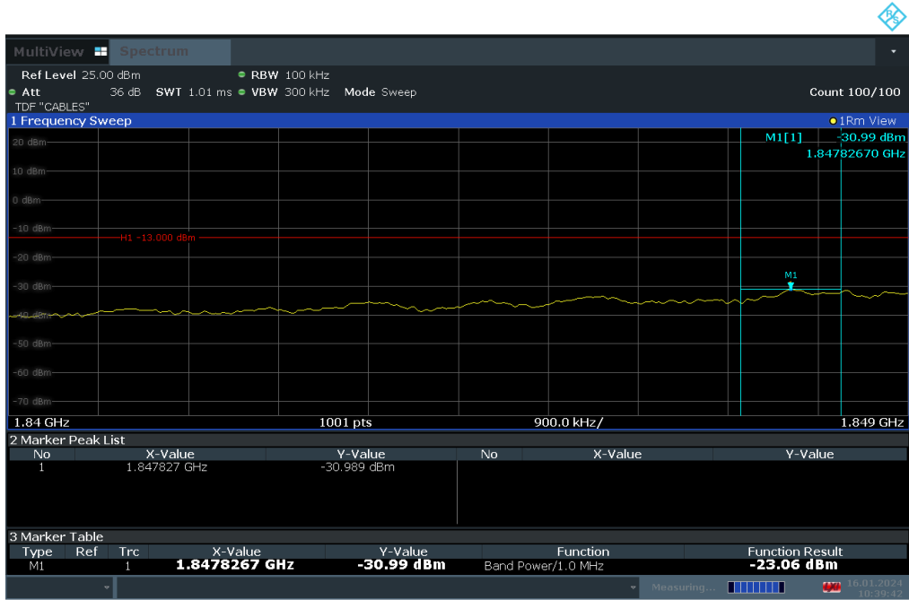
Plot 7-110. Extended Lower Band Edge Plot (LTE Band 25 – 15MHz QPSK – Full RB Configuration)
