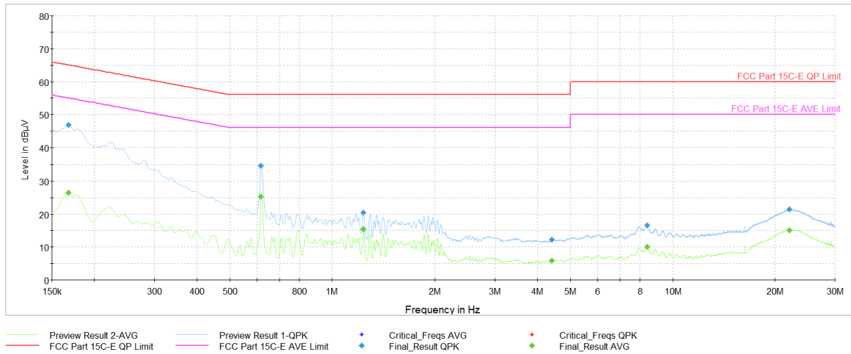
Plot 7-611. AC Line Conducted Plot with CDD 11ax - SU Ch.6 (L1, with Laptop)
