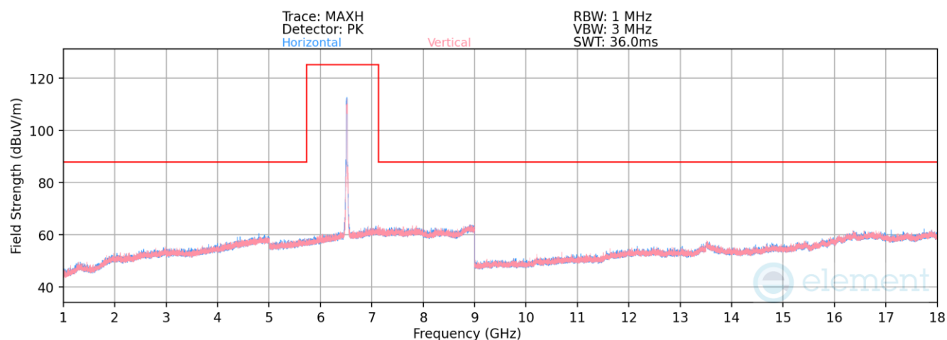
Plot 7-1638. Radiated Spurious Emissions above 1GHz Antenna 2a (802.11ax – Ch. 113 – RU242)
