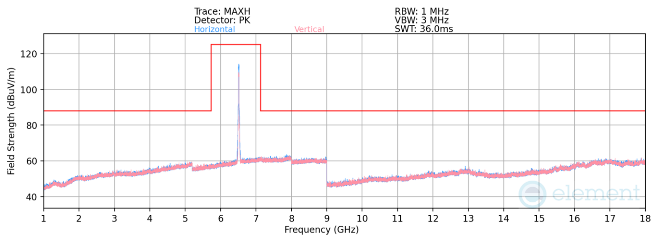
Plot 7-1667. Radiated Spurious Emissions above 1GHz SDM Primary (802.11ax – Ch. 113 – RU242)
