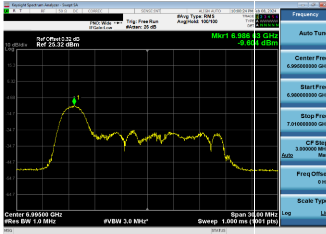
Plot 7-706. LPI Power Spectral Density Plot SDM Primary Antenna 4a (20MHz 802.11ax RU26 (UNII Band 8) – Ch. 209)
