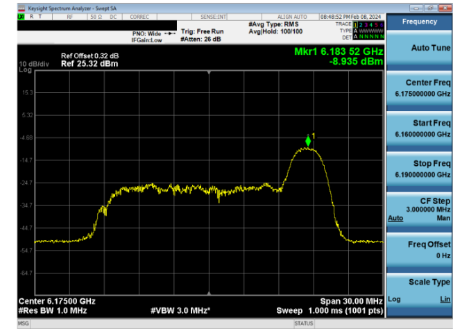
Plot 7-741. LPI Power Spectral Density Plot SDM Diversity Antenna 4a (20MHz 802.11ax RU26 (UNII Band 5) – Ch. 45)
