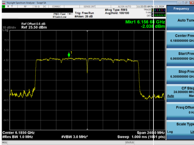
Plot 7-383. SP Power Spectral Density Plot CDD Diversity Antenna 4a (160MHz 802.11ax RU996x2 (UNII Band 5) – Ch. 47)
