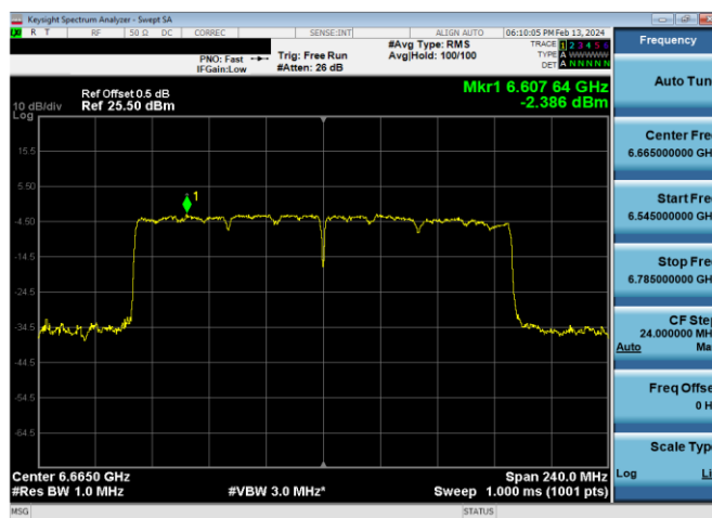
Plot 7-416. SP Power Spectral Density Plot CDD Diversity Antenna 2a (160MHz 802.11ax RU996x2 (UNII Band 7) – Ch. 143)
