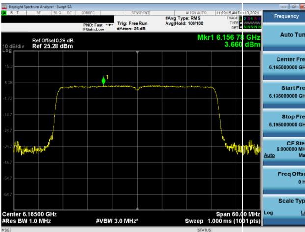
Plot 7-367. SP Power Spectral Density Plot CDD Diversity Antenna 4a (40MHz 802.11ax RU484 (UNII Band 5) – Ch. 43)
