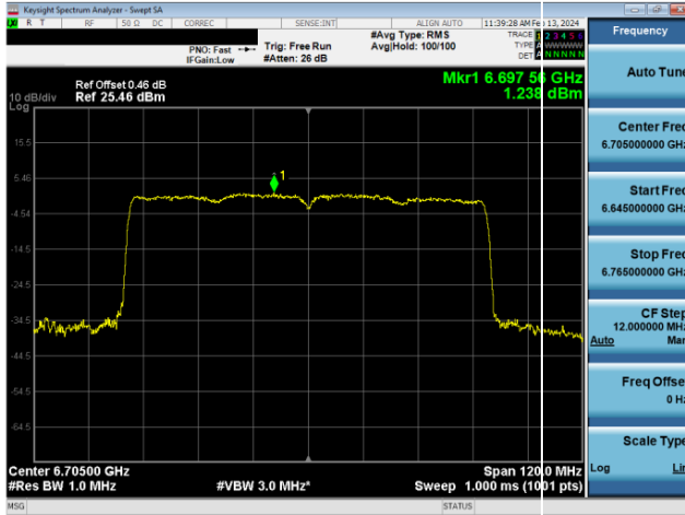
Plot 7-407. SP Power Spectral Density Plot CDD Diversity Antenna 4a (80MHz 802.11ax RU996 (UNII Band 7) – Ch. 151)
