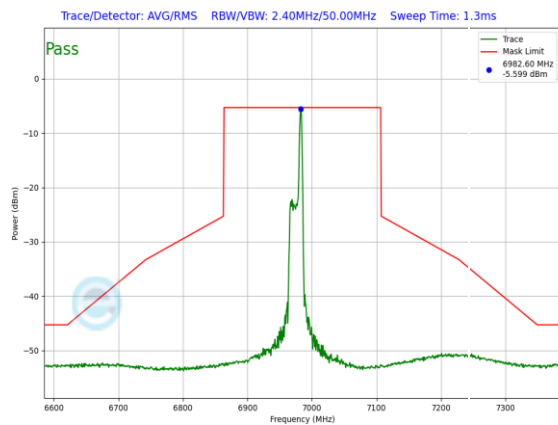
Plot 7-1214. LPI In-Band Emission Plot Antenna 3a (160MHz 802.11ax RU26 (UNII Band 8) – Ch. 207)
