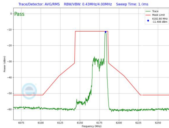
Plot 7-1293. LPI In-Band Emission Plot SDM Primary Antenna 3c (40MHz 802.11ax RU26 (UNII Band 5) – Ch. 43)
