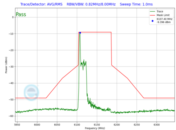
Plot 7-1297. LPI In-Band Emission Plot SDM Primary Antenna 3c (80MHz 802.11ax RU26 (UNII Band 5) – Ch. 39)
