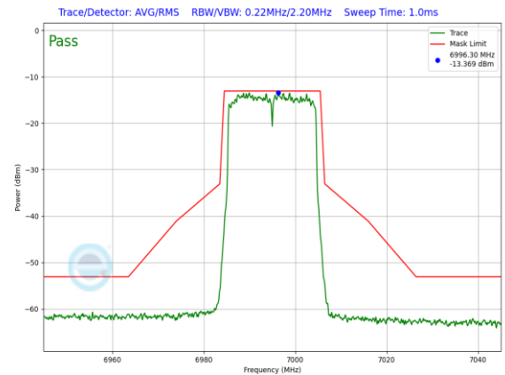
Plot 7-1204. LPI In-Band Emission Plot Antenna 3a (20MHz 802.11ax RU242 (UNII Band 8) – Ch. 209)
