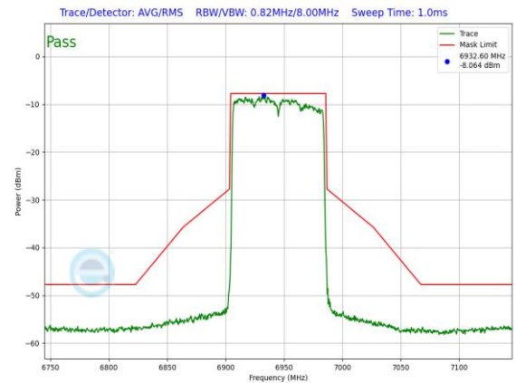
Plot 7-1212. LPI In-Band Emission Plot Antenna 3a (80MHz 802.11ax RU996 (UNII Band 8) – Ch. 199)
