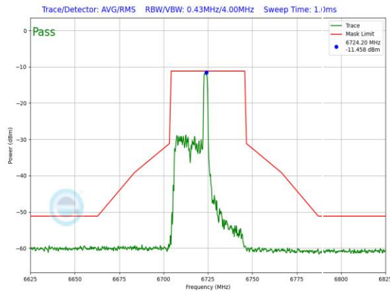
Plot 7-1190. LPI In-Band Emission Plot Antenna 3a (40MHz 802.11ax RU26 (UNII Band 7) – Ch. 155)
