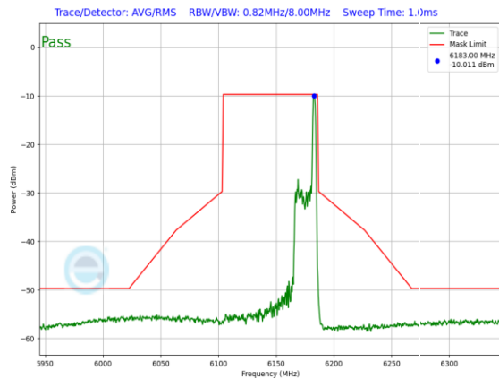
Plot 7-1301. LPI In-Band Emission Plot SDM Primary Antenna 3c (80MHz 802.11ax RU26 (UNII Band 5) – Ch. 39)
