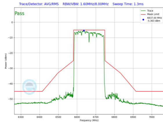
Plot 7-1200. LPI In-Band Emission Plot Antenna 3a (160MHz 802.11ax RU996x2 (UNII Band 7) – Ch. 143)
