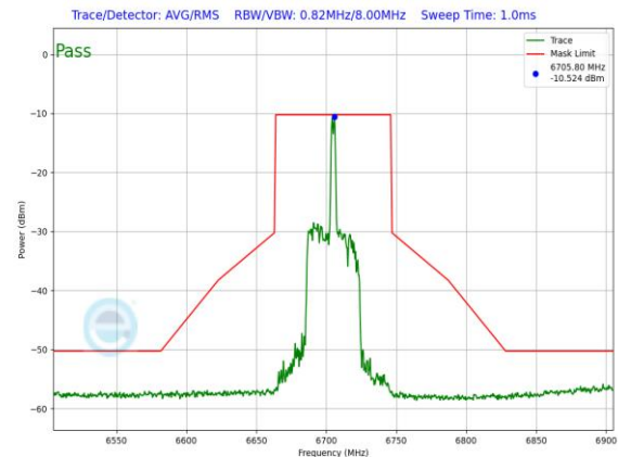
Plot 7-1194. LPI In-Band Emission Plot Antenna 3a (80MHz 802.11ax RU26 (UNII Band 7) – Ch. 151)
