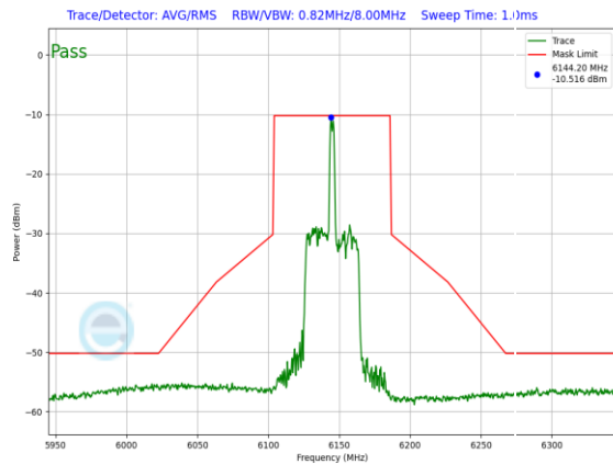
Plot 7-1299. LPI In-Band Emission Plot SDM Primary Antenna 3c (80MHz 802.11ax RU26 (UNII Band 5) – Ch. 39)
