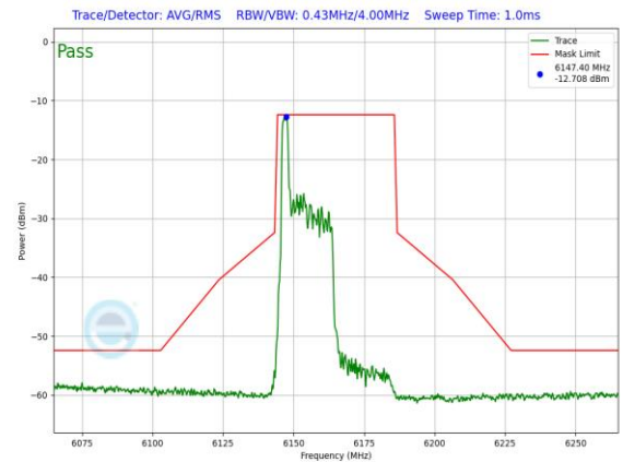
Plot 7-1290. LPI In-Band Emission Plot SDM Primary Antenna 3a (40MHz) 802.11ax RU26 (UNII Band 5) – Ch. 43)
