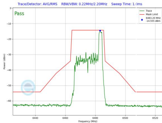
Plot 7-1318. LPI In-Band Emission Plot SDM Primary Antenna 3a (20MHz 802.11ax RU26 (UNII Band 6) – Ch. 105)
