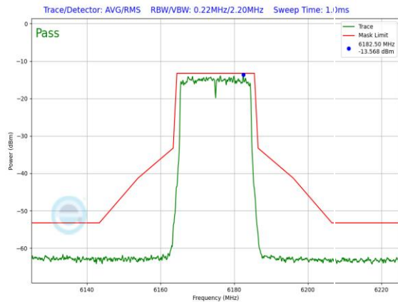
Plot 7-1287. LPI In-Band Emission Plot SDM Primary Antenna 3c (20MHz) 802.11ax RU242 (UNII Band 5) – Ch. 45)
