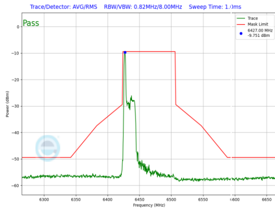
Plot 7-1329. LPI In-Band Emission Plot SDM Primary Antenna 3c (80MHz 802.11ax RU26 (UNII Band 6) – Ch. 103)
