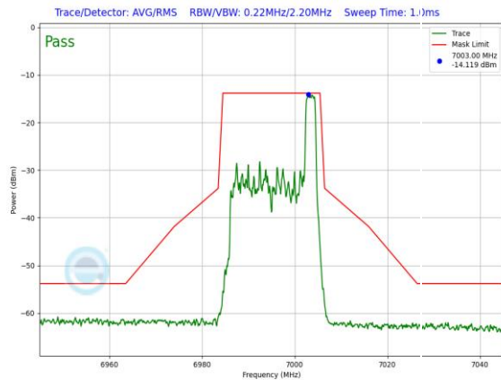
Plot 7-1203. LPI In-Band Emission Plot Antenna 3a (20MHz 802.11ax RU26 (UNII Band 8) – Ch. 209)
