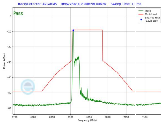
Plot 7-1209. LPI In-Band Emission Plot Antenna 3a (80MHz 802.11ax RU26 (UNII Band 8) – Ch. 199)
