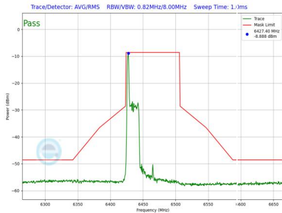
Plot 7-1330. LPI In-Band Emission Plot SDM Primary Antenna 3a (80MHz 802.11ax RU26 (UNII Band 6) – Ch. 103)
