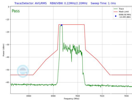
Plot 7-1201. LPI In-Band Emission Plot Antenna 3a (20MHz 802.11ax RU26 (UNII Band 8) – Ch. 209)
