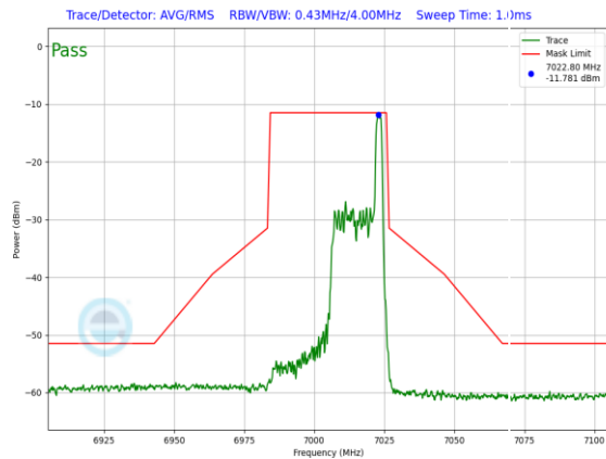
Plot 7-1207. LPI In-Band Emission Plot Antenna 3a (40MHz 802.11ax RU26 (UNII Band 8) – Ch. 211)
