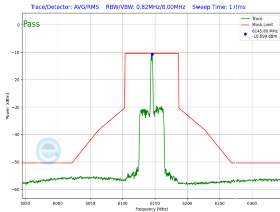
Plot 7-1300. LPI In-Band Emission Plot SDM Primary Antenna 3a (80MHz 802.11ax RU26 (UNII Band 5) – Ch. 39)
