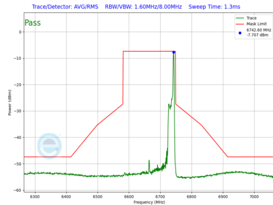
Plot 7-1199. LPI In-Band Emission Plot Antenna 3a (160MHz 802.11ax RU26 (UNII Band 7) – Ch. 143)
