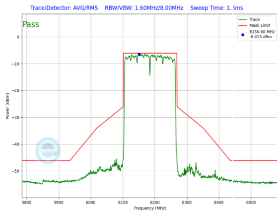
Plot 7-1312. LPI In-Band Emission Plot SDM Primary Antenna 3a (160MHz 802.11ax RU996x2 (UNII Band 5) – Ch. 47)
