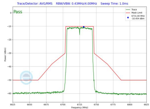
Plot 7-1192. LPI In-Band Emission Plot Antenna 3a (40MHz 802.11ax RU484 (UNII Band 7) – Ch. 155)
