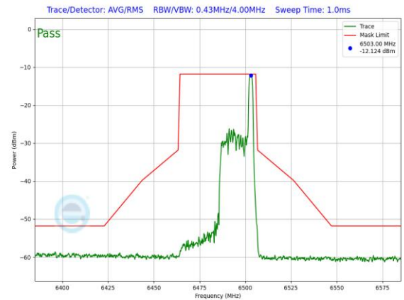
Plot 7-1326. LPI In-Band Emission Plot SDM Primary Antenna 3a (40MHz 802.11ax RU26 (UNII Band 6) – Ch. 107)
