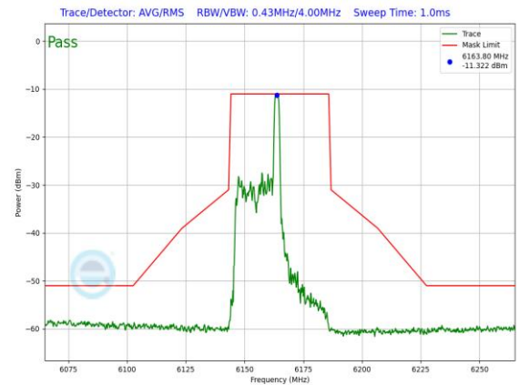
Plot 7-1291. LPI In-Band Emission Plot SDM Primary Antenna 3c (40MHz) 802.11ax RU26 (UNII Band 5) – Ch. 43)
