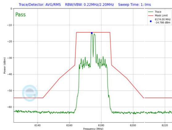
Plot 7-1283. LPI In-Band Emission Plot SDM Primary Antenna 3c (20MHz 802.11ax RU26 (UNII Band 5) – Ch. 45)
