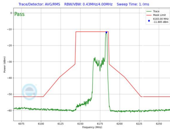
Plot 7-1294. LPI In-Band Emission Plot SDM Primary Antenna 3a (40MHz 802.11ax RU26 (UNII Band 5) – Ch. 43)
