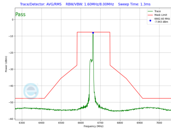
Plot 7-1198. LPI In-Band Emission Plot Antenna 3a (160MHz 802.11ax RU26 (UNII Band 7) – Ch. 143)
