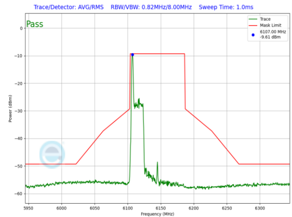
Plot 7-1298. LPI In-Band Emission Plot SDM Primary Antenna 3a (80MHz 802.11ax RU26 (UNII Band 5) – Ch. 39)
