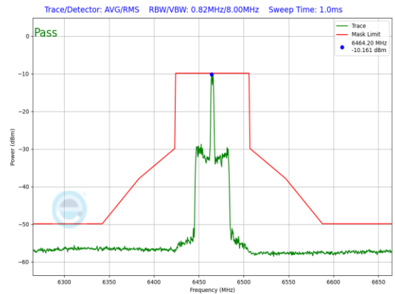
Plot 7-1332. LPI In-Band Emission Plot SDM Primary Antenna 3a (80MHz 802.11ax RU26 (UNII Band 6) – Ch. 103)
