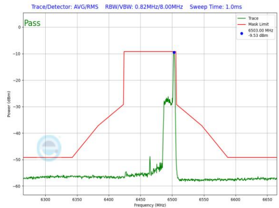
Plot 7-1334. LPI In-Band Emission Plot SDM Primary Antenna 3a (80MHz 802.11ax RU26 (UNII Band 6) – Ch. 103)
