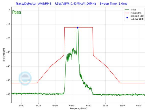
Plot 7-1323. LPI In-Band Emission Plot SDM Primary Antenna 3c (40MHz 802.11ax RU26 (UNII Band 6) – Ch. 107)
