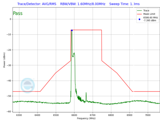
Plot 7-1197. LPI In-Band Emission Plot Antenna 3a (160MHz 802.11ax RU26 (UNII Band 7) – Ch. 143)
