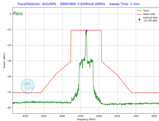
Plot 7-1331. LPI In-Band Emission Plot SDM Primary Antenna 3c (80MHz 802.11ax RU26 (UNII Band 6) – Ch. 103)
