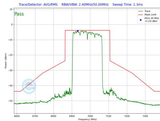
Plot 7-1216. LPI In-Band Emission Plot Antenna 3a (160MHz 802.11ax RU996x2 (UNII Band 8) – Ch. 207)
