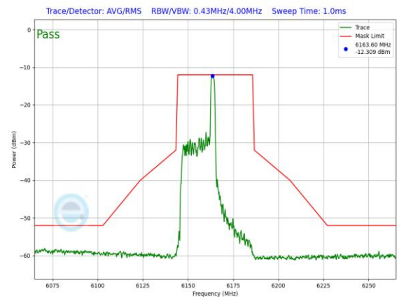
Plot 7-1292. LPI In-Band Emission Plot SDM Primary Antenna 3a (40MHz) 802.11ax RU26 (UNII Band 5) – Ch. 43)
