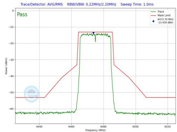
Plot 7-1320. LPI In-Band Emission Plot SDM Primary Antenna 3a (20MHz 802.11ax RU242 (UNII Band 6) – Ch. 105)
