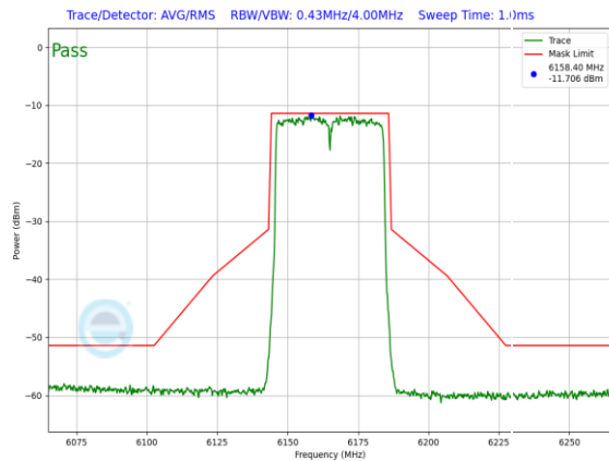
Plot 7-1295. LPI In-Band Emission Plot SDM Primary Antenna 3c (40MHz 802.11ax RU484 (UNII Band 5) – Ch. 43)
