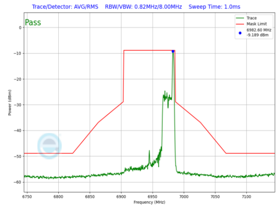
Plot 7-1211. LPI In-Band Emission Plot Antenna 3a (80MHz 802.11ax RU26 (UNII Band 8) – Ch. 199)
