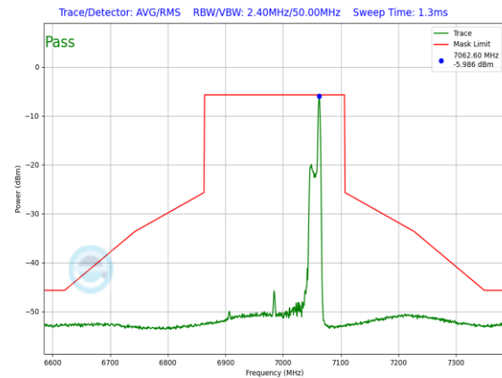
Plot 7-1215. LPI In-Band Emission Plot Antenna 3a (160MHz 802.11ax RU26 (UNII Band 8) – Ch. 207)
