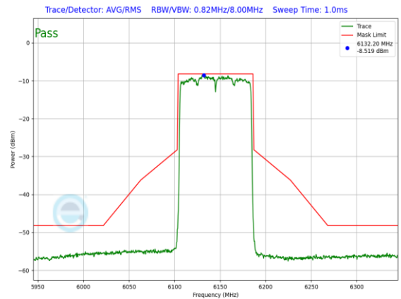
Plot 7-1304. LPI In-Band Emission Plot SDM Primary Antenna 3a (80MHz 802.11ax RU996 (UNII Band 5) – Ch. 39)
