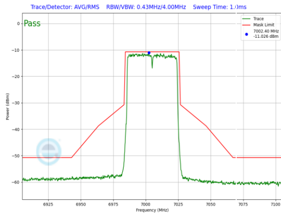
Plot 7-1208. LPI In-Band Emission Plot Antenna 3a (40MHz 802.11ax RU484 (UNII Band 8) – Ch. 211)
