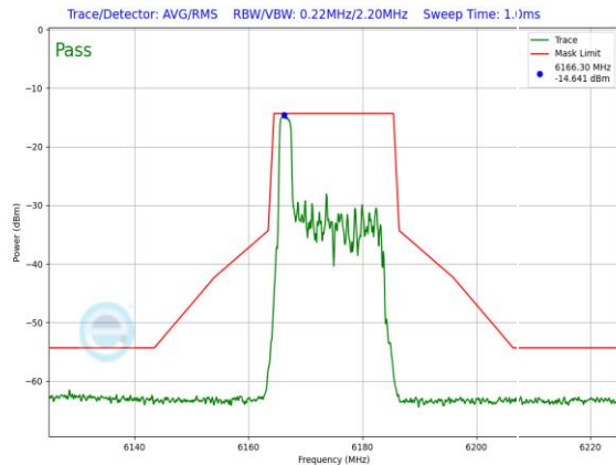
Plot 7-1282. LPI In-Band Emission Plot SDM Primary Antenna 3a (20MHz 802.11ax RU26 (UNII Band 5) – Ch. 45)
