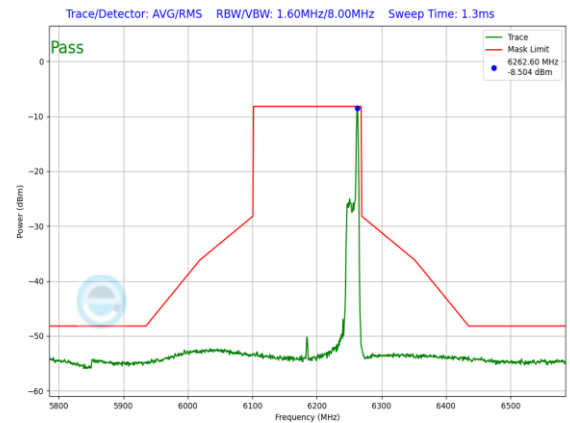
Plot 7-1310. LPI In-Band Emission Plot SDM Primary Antenna 3a (160MHz 802.11ax RU26 (UNII Band 5) – Ch. 47)
