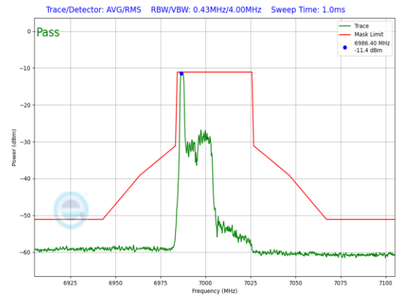
Plot 7-1205. LPI In-Band Emission Plot Antenna 3a (40MHz 802.11ax RU26 (UNII Band 8) – Ch. 211)
