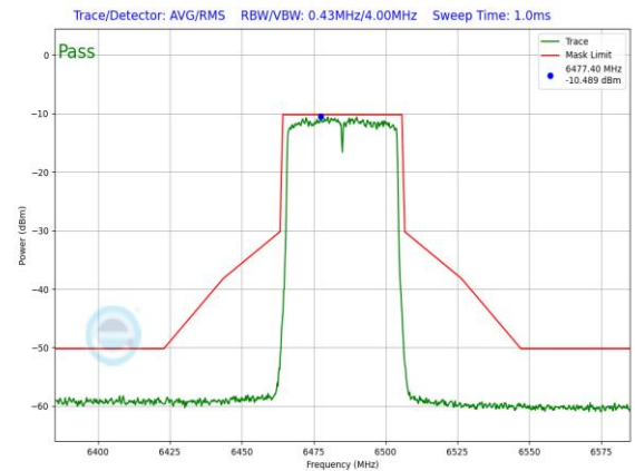
Plot 7-1328. LPI In-Band Emission Plot SDM Primary Antenna 3a (40MHz 802.11ax RU484 (UNII Band 6) – Ch. 107)
