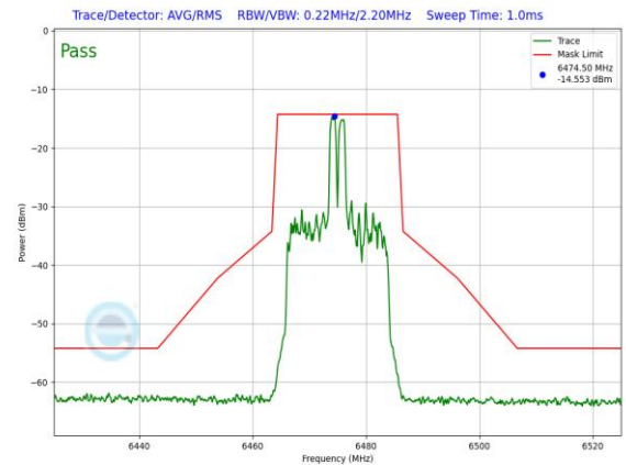
Plot 7-1316. LPI In-Band Emission Plot SDM Primary Antenna 3a (20MHz 802.11ax RU26 (UNII Band 6) – Ch. 105)
