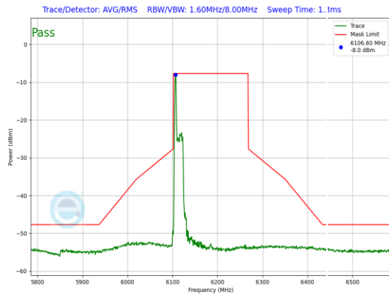
Plot 7-1305. LPI In-Band Emission Plot SDM Primary Antenna 3c (160MHz 802.11ax RU26 (UNII Band 5) – Ch. 47)
