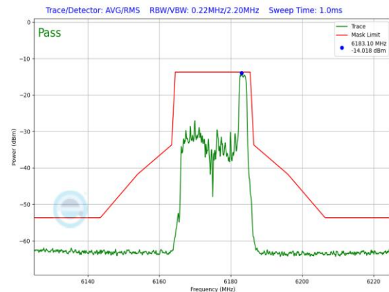
Plot 7-1286. LPI In-Band Emission Plot SDM Primary Antenna 3a (20MHz 802.11ax RU26 (UNII Band 5) – Ch. 45)
