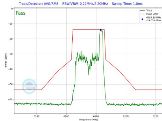
Plot 7-1285. LPI In-Band Emission Plot SDM Primary Antenna 3c (20MHz 802.11ax RU26 (UNII Band 5) – Ch. 45)
