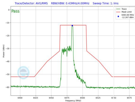
Plot 7-1324. LPI In-Band Emission Plot SDM Primary Antenna 3a (40MHz 802.11ax RU26 (UNII Band 6) – Ch. 107)
