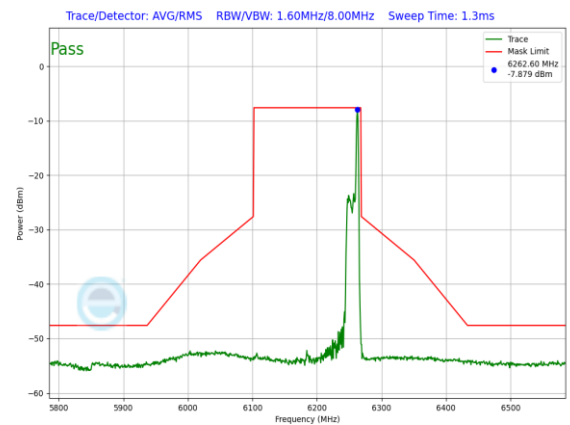
Plot 7-1309. LPI In-Band Emission Plot SDM Primary Antenna 3c (160MHz 802.11ax RU26 (UNII Band 5) – Ch. 47)
