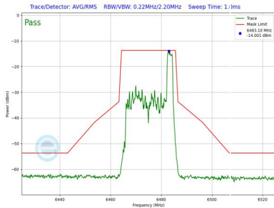
Plot 7-1317. LPI In-Band Emission Plot SDM Primary Antenna 3c (20MHz 802.11ax RU26 (UNII Band 6) – Ch. 105)
