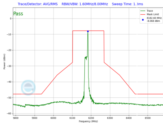
Plot 7-1307. LPI In-Band Emission Plot SDM Primary Antenna 3c (160MHz 802.11ax RU26 (UNII Band 5) – Ch. 47)
