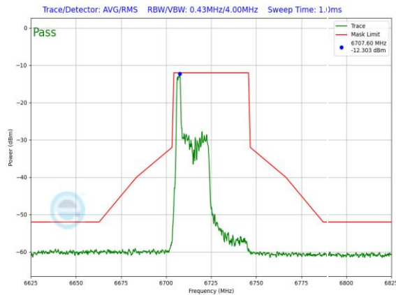
Plot 7-1189. LPI In-Band Emission Plot Antenna 3a (40MHz 802.11ax RU26 (UNII Band 7) – Ch. 155)
