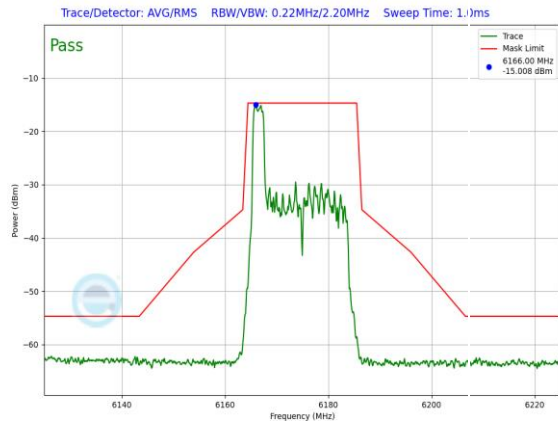
Plot 7-1281. LPI In-Band Emission Plot SDM Primary Antenna 3c (20MHz 802.11ax RU26 (UNII Band 5) – Ch. 45)
