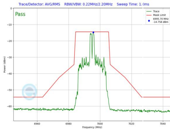
Plot 7-1202. LPI In-Band Emission Plot Antenna 3a (20MHz 802.11ax RU26 (UNII Band 8) – Ch. 209)
