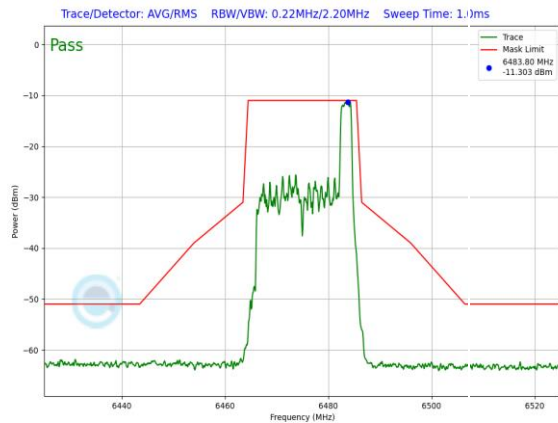
Plot 7-1235. LPI In-Band Emission Plot Antenna 1b (20MHz 802.11ax RU26 (UNII Band 6) – Ch. 105)
