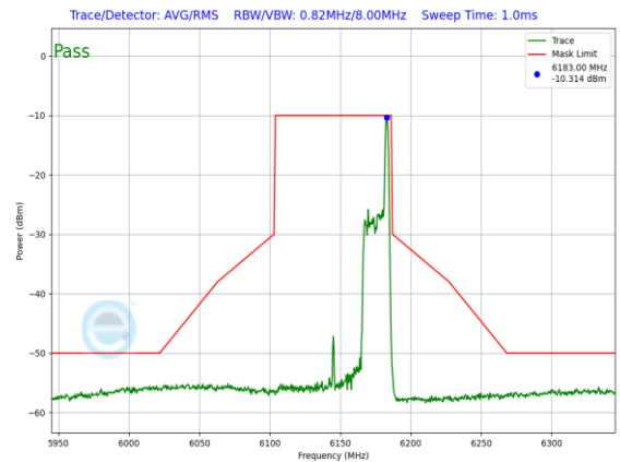
Plot 7-1302. LPI In-Band Emission Plot SDM Primary Antenna 3a (80MHz 802.11ax RU26 (UNII Band 5) – Ch. 39)
