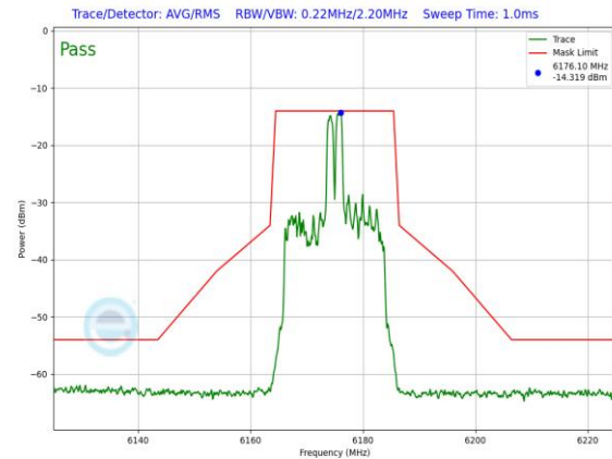
Plot 7-1284. LPI In-Band Emission Plot SDM Primary Antenna 3a (20MHz 802.11ax RU26 (UNII Band 5) – Ch. 45)
