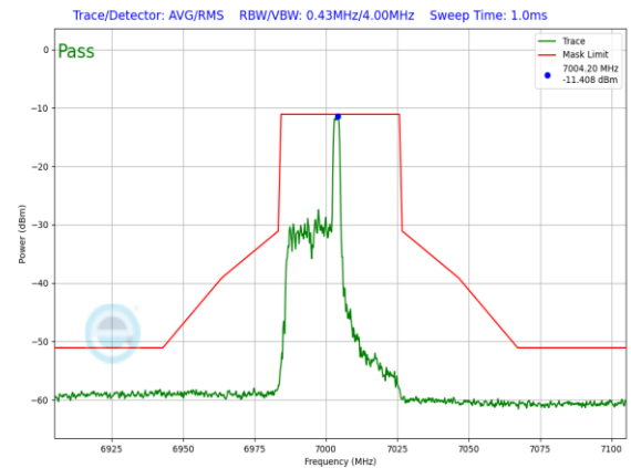
Plot 7-1206. LPI In-Band Emission Plot Antenna 3a (40MHz 802.11ax RU26 (UNII Band 8) – Ch. 211)
