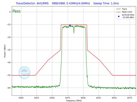
Plot 7-1327. LPI In-Band Emission Plot SDM Primary Antenna 3c (40MHz 802.11ax RU484 (UNII Band 6) – Ch. 107)
