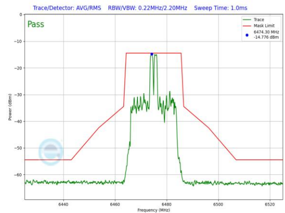
Plot 7-1315. LPI In-Band Emission Plot SDM Primary Antenna 3c (20MHz 802.11ax RU26 (UNII Band 6) – Ch. 105)
