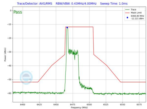
Plot 7-1322. LPI In-Band Emission Plot SDM Primary Antenna 3a (40MHz 802.11ax RU26 (UNII Band 6) – Ch. 107)
