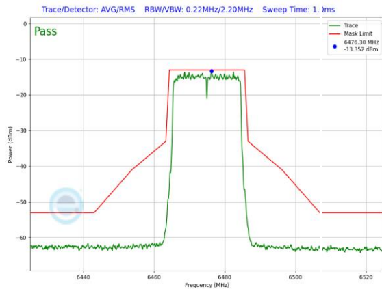
Plot 7-1319. LPI In-Band Emission Plot SDM Primary Antenna 3c (20MHz 802.11ax RU242 (UNII Band 6) – Ch. 105)
