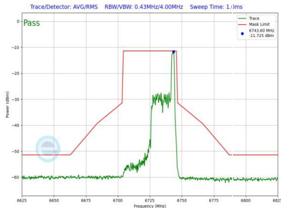
Plot 7-1191. LPI In-Band Emission Plot Antenna 3a (40MHz 802.11ax RU26 (UNII Band 7) – Ch. 155)
