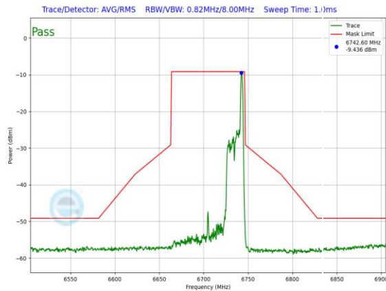
Plot 7-1195. LPI In-Band Emission Plot Antenna 3a (80MHz 802.11ax RU26 (UNII Band 7) – Ch. 151)
