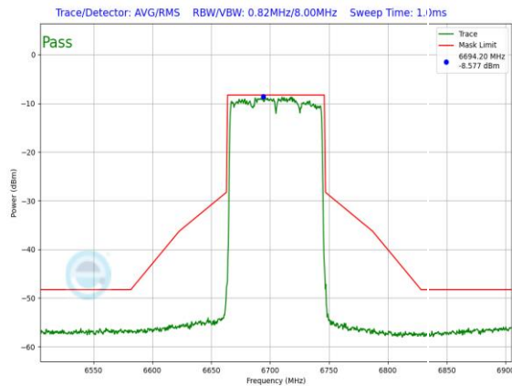
Plot 7-1196. LPI In-Band Emission Plot Antenna 3a (80MHz 802.11ax RU996 (UNII Band 7) – Ch. 151)
