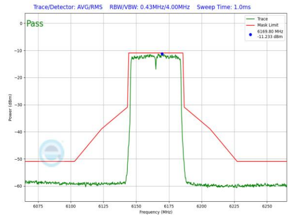
Plot 7-1296. LPI In-Band Emission Plot SDM Primary Antenna 3a (40MHz 802.11ax RU484 (UNII Band 5) – Ch. 43)
