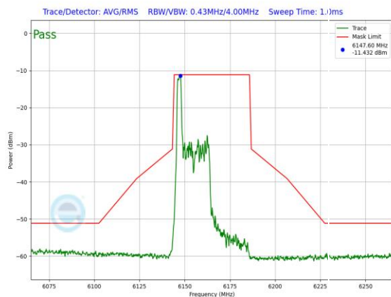
Plot 7-1289. LPI In-Band Emission Plot SDM Primary Antenna 3c (40MHz) 802.11ax RU26 (UNII Band 5) – Ch. 43)
