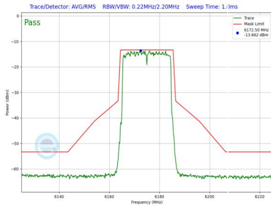
Plot 7-1288. LPI In-Band Emission Plot SDM Primary Antenna 3a (20MHz) 802.11ax RU242 (UNII Band 5) – Ch. 45)
