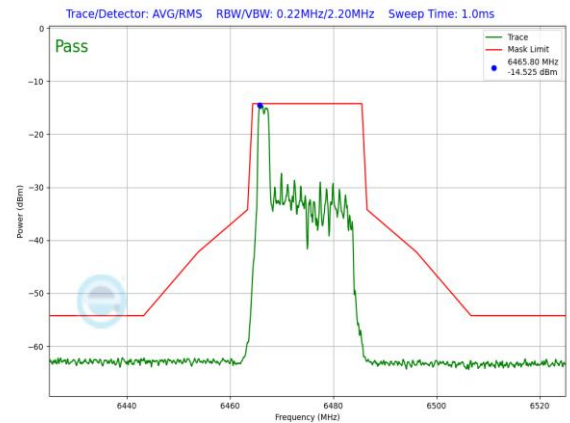
Plot 7-1314. LPI In-Band Emission Plot SDM Primary Antenna 3a (20MHz 802.11ax RU26 (UNII Band 6) – Ch. 105)
