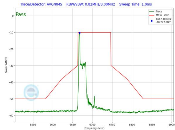
Plot 7-1193. LPI In-Band Emission Plot Antenna 3a (80MHz 802.11ax RU26 (UNII Band 7) – Ch. 151)
