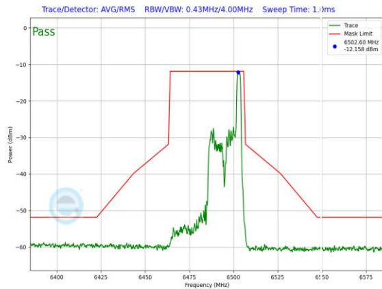
Plot 7-1325. LPI In-Band Emission Plot SDM Primary Antenna 3c (40MHz 802.11ax RU26 (UNII Band 6) – Ch. 107)
