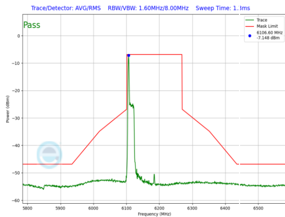
Plot 7-1306. LPI In-Band Emission Plot SDM Primary Antenna 3a (160MHz 802.11ax RU26 (UNII Band 5) – Ch. 47)
