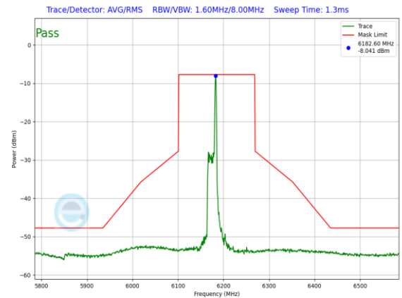
Plot 7-1308. LPI In-Band Emission Plot SDM Primary Antenna 3a (160MHz 802.11ax RU26 (UNII Band 5) – Ch. 47)
