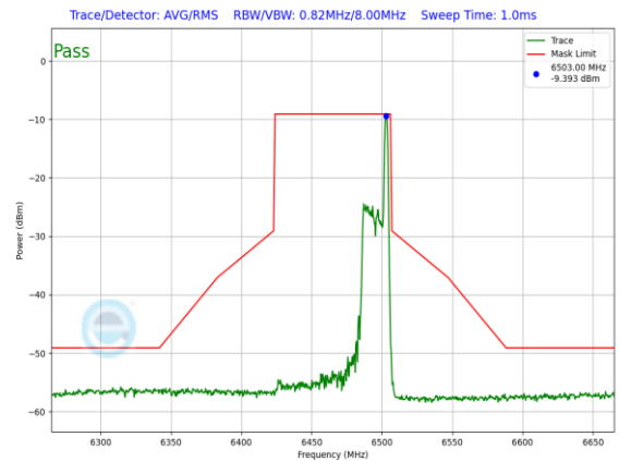
Plot 7-1333. LPI In-Band Emission Plot SDM Primary Antenna 3c (80MHz 802.11ax RU26 (UNII Band 6) – Ch. 103)
