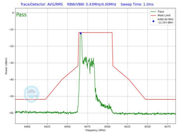
Plot 7-1321. LPI In-Band Emission Plot SDM Primary Antenna 3c (40MHz 802.11ax RU26 (UNII Band 6) – Ch. 107)
