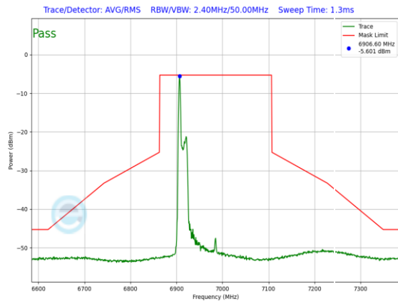
Plot 7-1213. LPI In-Band Emission Plot Antenna 3a (160MHz 802.11ax RU26 (UNII Band 8) – Ch. 207)
