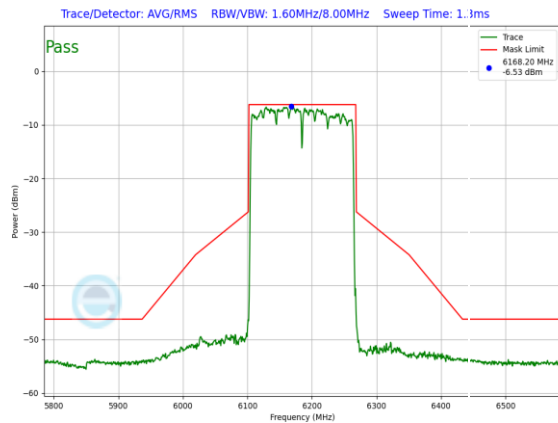
Plot 7-1311. LPI In-Band Emission Plot SDM Primary Antenna 3c (160MHz 802.11ax RU996x2 (UNII Band 5) – Ch. 47)
