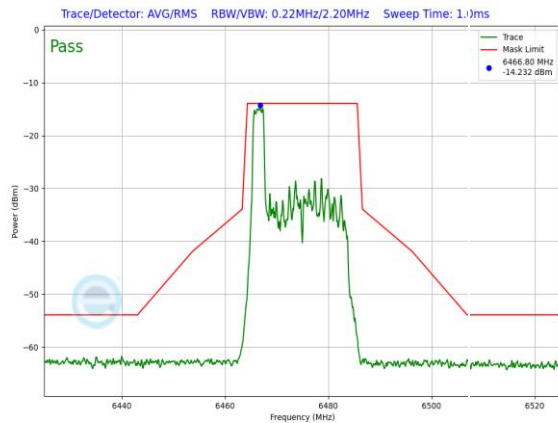
Plot 7-1313. LPI In-Band Emission Plot SDM Primary Antenna 3c (20MHz 802.11ax RU26 (UNII Band 6) – Ch. 105)
