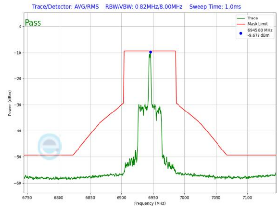
Plot 7-1210. LPI In-Band Emission Plot Antenna 3a (80MHz 802.11ax RU26 (UNII Band 8) – Ch. 199)
