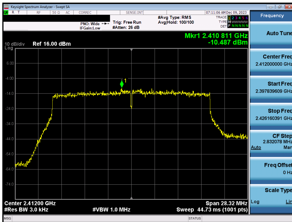
Plot 7-134. Power Spectral Density Plot CDD Antenna 1a (802.11ax (SU - 2.4GHz) – Ch. 1) – MCS2
