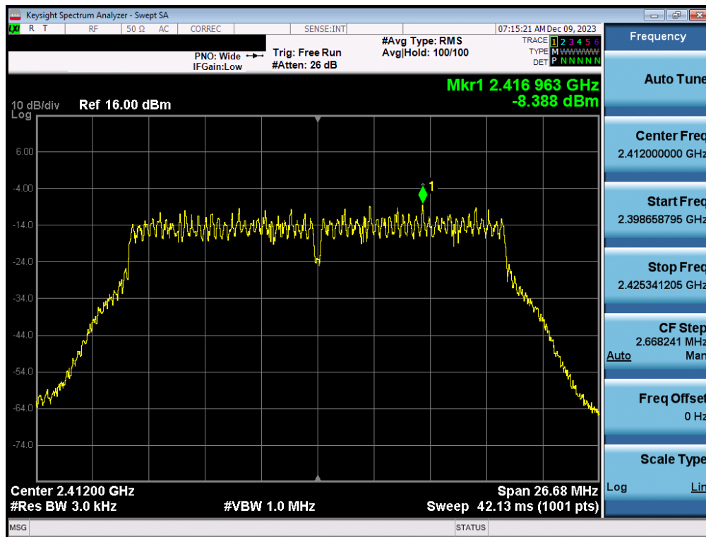
Plot 7-164. Power Spectral Density Plot CDD Antenna 1a(802.11n (2.4GHz) – Ch. 1) – MCS15
