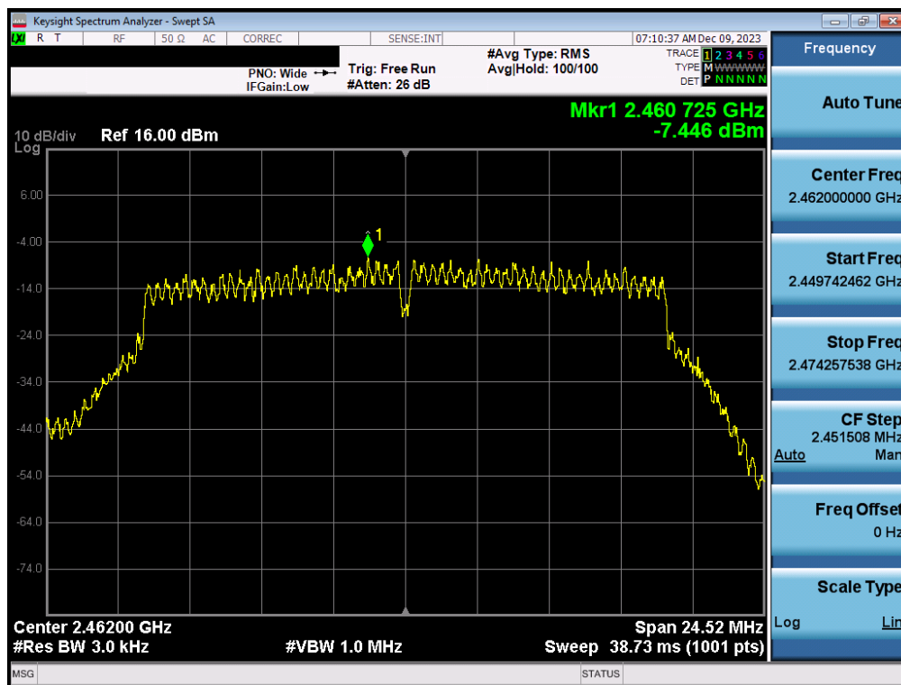
Plot 7-132. Power Spectral Density Plot CDD Antenna 1a (802.11n (2.4GHz) – Ch. 11) – MCS10
