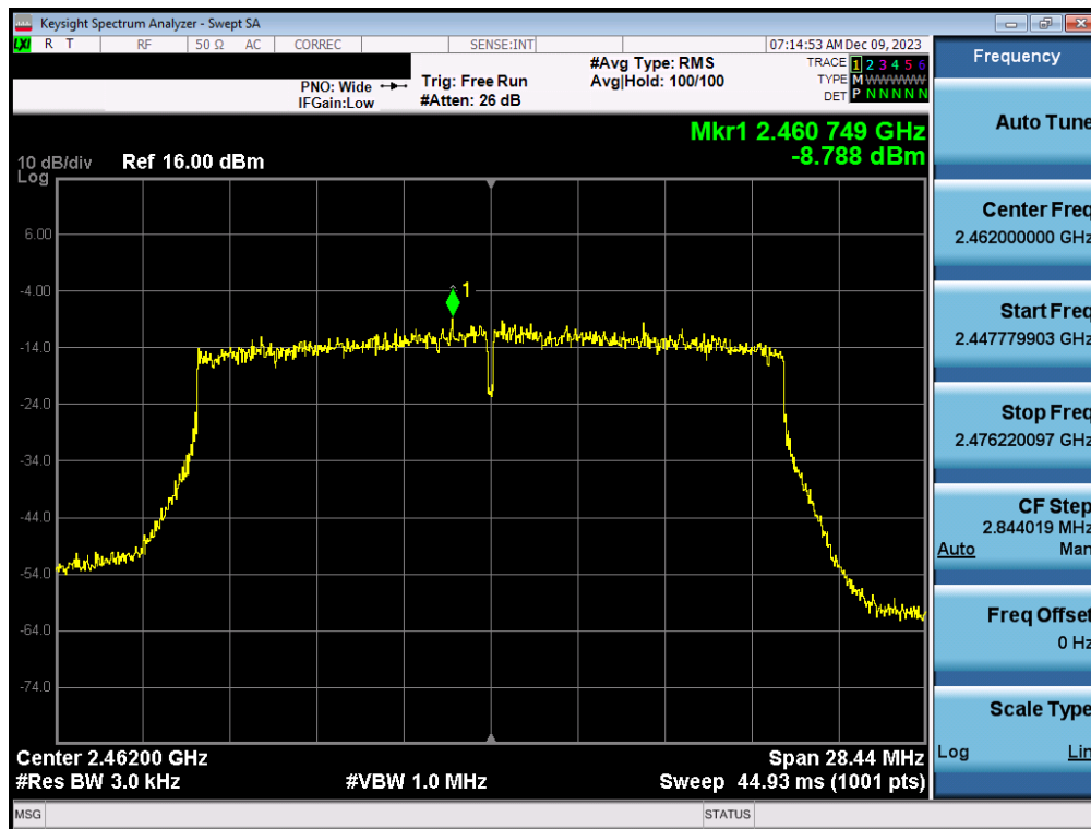
Plot 7-156. Power Spectral Density Plot CDD Antenna 1a (802.11ax (SU - 2.4GHz) – Ch. 11) – MCS4
