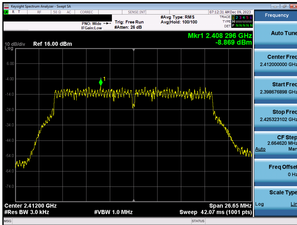
Plot 7-146. Power Spectral Density Plot CDD Antenna 1a(802.11n (2.4GHz) – Ch. 1) – MCS12
