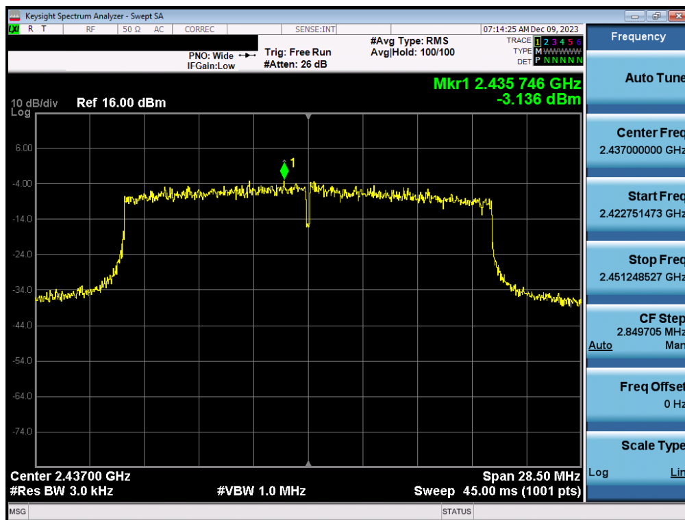
Plot 7-154. Power Spectral Density Plot CDD Antenna 1a (802.11ax (SU - 2.4GHz) – Ch. 6) – MCS4
