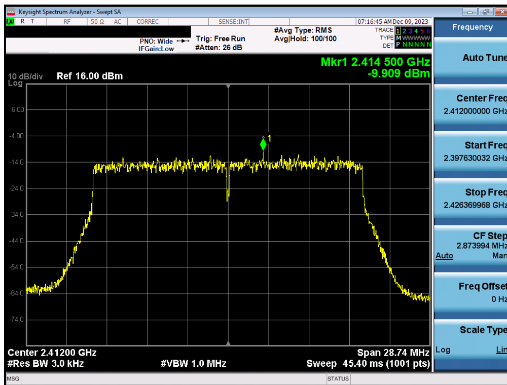
Plot 7-170. Power Spectral Density Plot CDD Antenna 1a (802.11ax (SU - 2.4GHz) – Ch. 1) – MCS9
