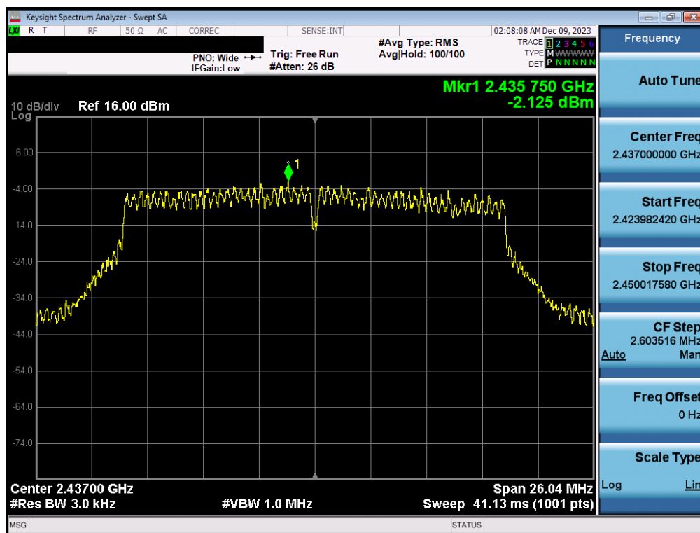
Plot 7-129. Power Spectral Density Plot CDD Antenna 3a(802.11n (2.4GHz) – Ch. 6) – MCS10
