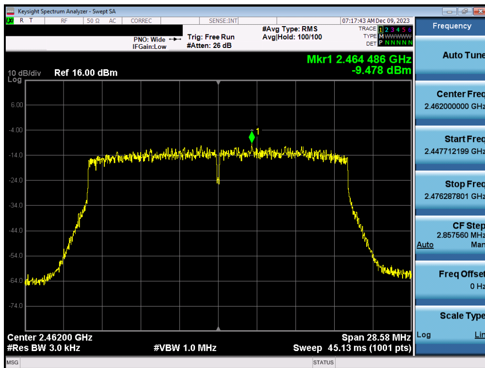
Plot 7-174. Power Spectral Density Plot CDD Antenna 1a (802.11ax (SU - 2.4GHz) – Ch. 11) – MCS9
