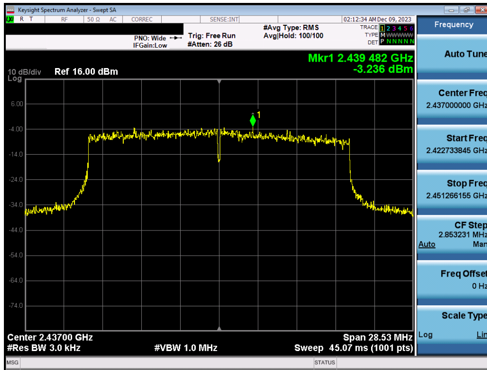
Plot 7-153. Power Spectral Density Plot CDD Antenna 3a (802.11ax (SU - 2.4GHz) – Ch. 6) – MCS4
