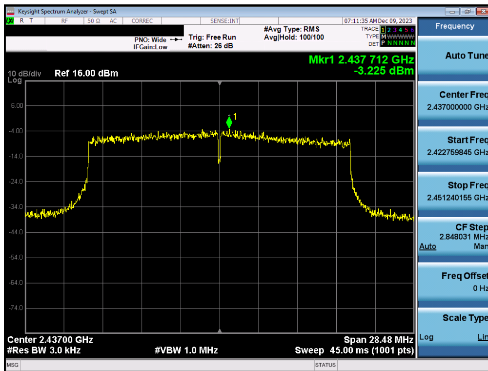
Plot 7-136. Power Spectral Density Plot CDD Antenna 1a (802.11ax (SU - 2.4GHz) – Ch. 6) – MCS2
