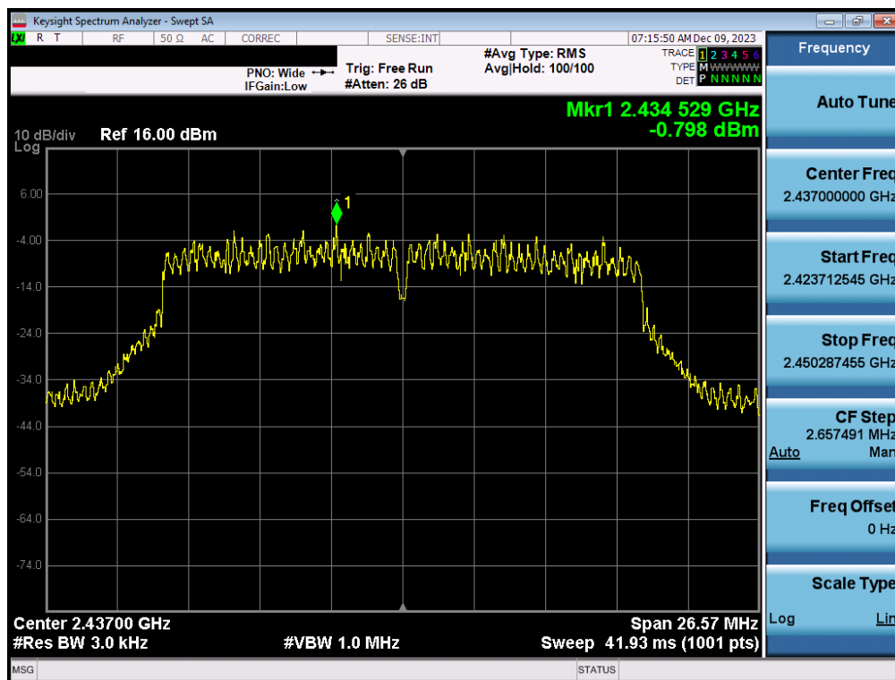
Plot 7-166. Power Spectral Density Plot CDD Antenna 1a(802.11n (2.4GHz) – Ch. 6) – MCS15
