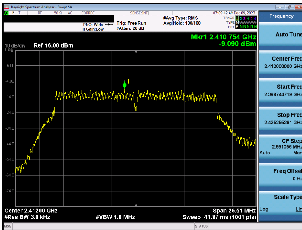
Plot 7-128. Power Spectral Density Plot CDD Antenna 1a(802.11n (2.4GHz) – Ch. 1) – MCS10
