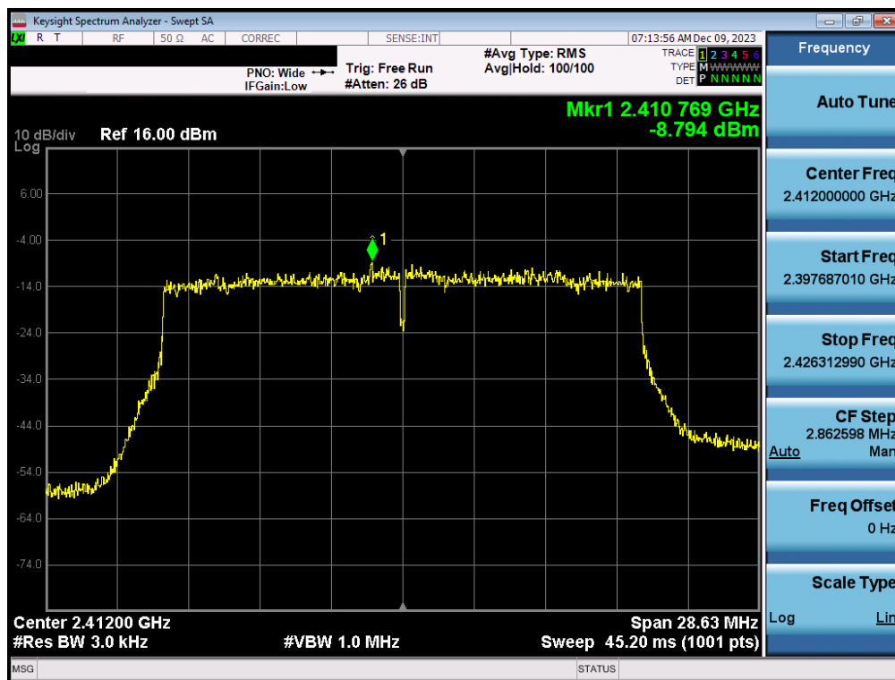
Plot 7-152. Power Spectral Density Plot CDD Antenna 1a (802.11ax (SU - 2.4GHz) – Ch. 1) – MCS4
