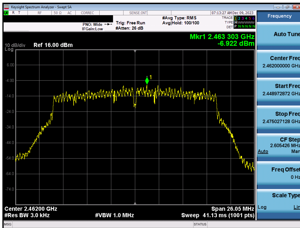
Plot 7-150. Power Spectral Density Plot CDD Antenna 1a (802.11n (2.4GHz) – Ch. 11) – MCS12
