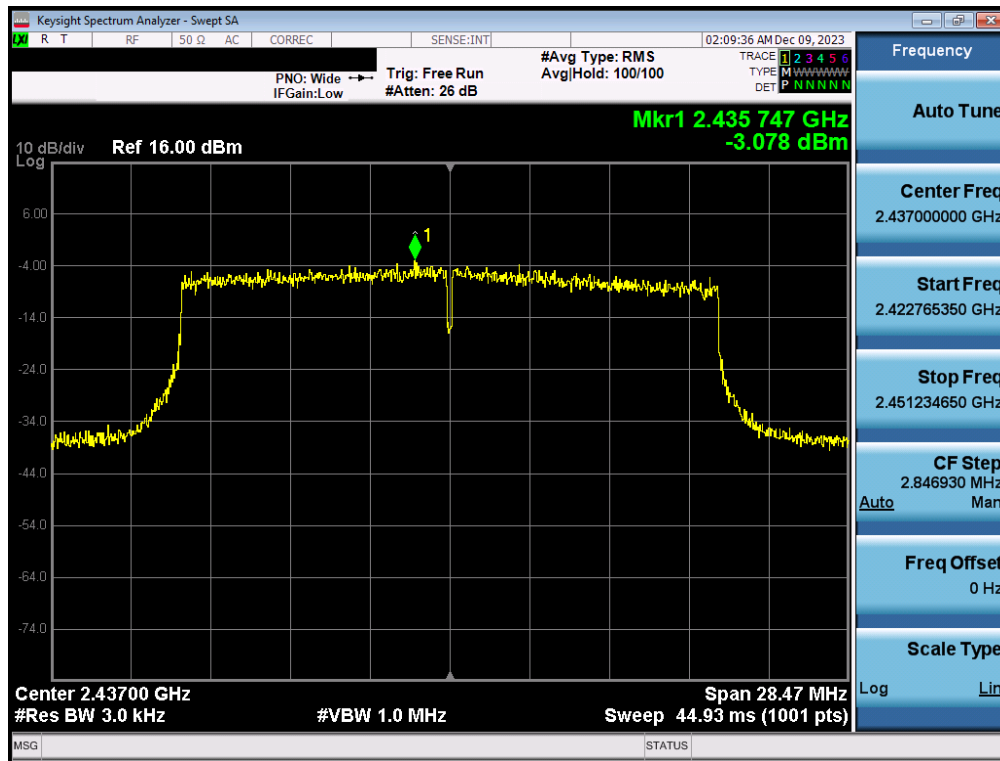
Plot 7-135. Power Spectral Density Plot CDD Antenna 3a (802.11ax (SU - 2.4GHz) – Ch. 6) – MCS2
