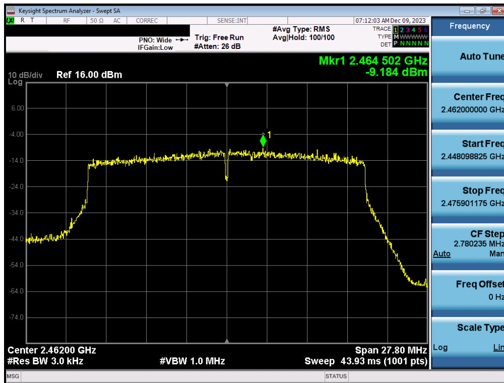
Plot 7-138. Power Spectral Density Plot CDD Antenna 1a (802.11ax (SU - 2.4GHz) – Ch. 11) – MCS2
