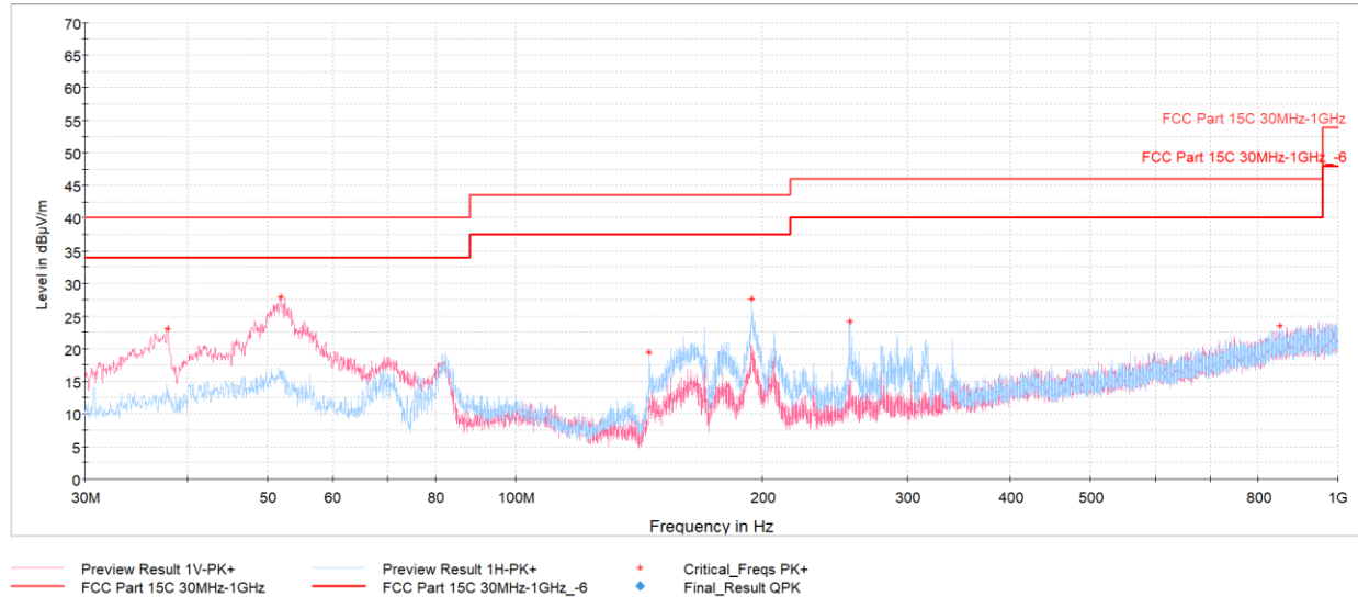
Plot 7-103. Radiated Spurious Emissions Below 1GHz TxBF (1Mbps, ePA – Ch.19, Pol. H & V, with AC/DC Adapter)
