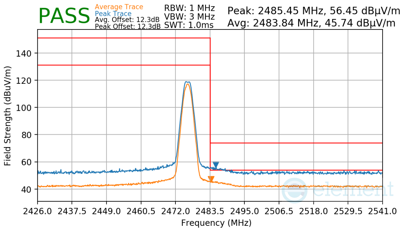
Plot 7-98. Radiated Restricted Upper Band Edge Measurement Antenna 1a (Average & Peak)
