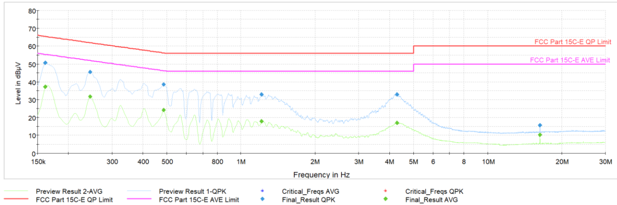
Plot 7-104. AC Line Conducted Plot with Bluetooth LE Tx BF (L1, 1Mbps ePA – Ch.19 with AC/DC Charger)
