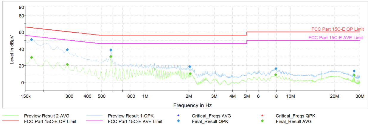
Plot 7-105. AC Line Conducted Plot with Bluetooth LE TxBF (N, 1Mbps ePA – Ch.19, with Laptop Charger)
