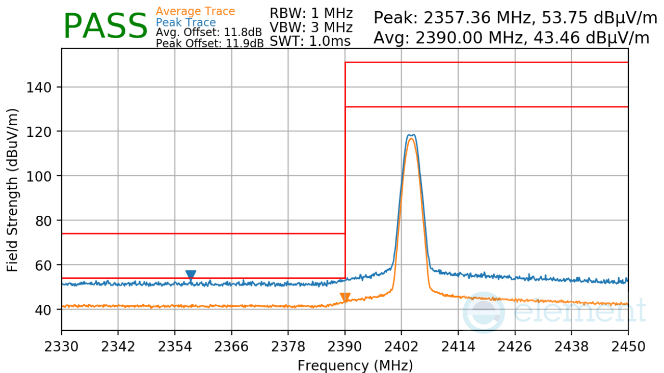
Plot 7-97. Radiated Restricted Lower Band Edge Measurement Antenna 1a (Average & Peak)
