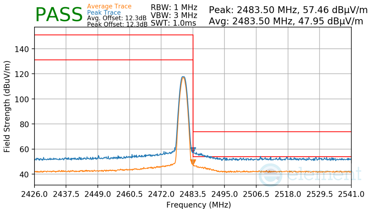
Plot 7-96. Radiated Restricted Upper Band Edge Measurement Antenna 1a (Average & Peak)
