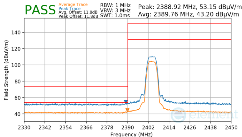
Plot 7-96. Radiated Restricted Lower Band Edge Measurement Antenna 1a
