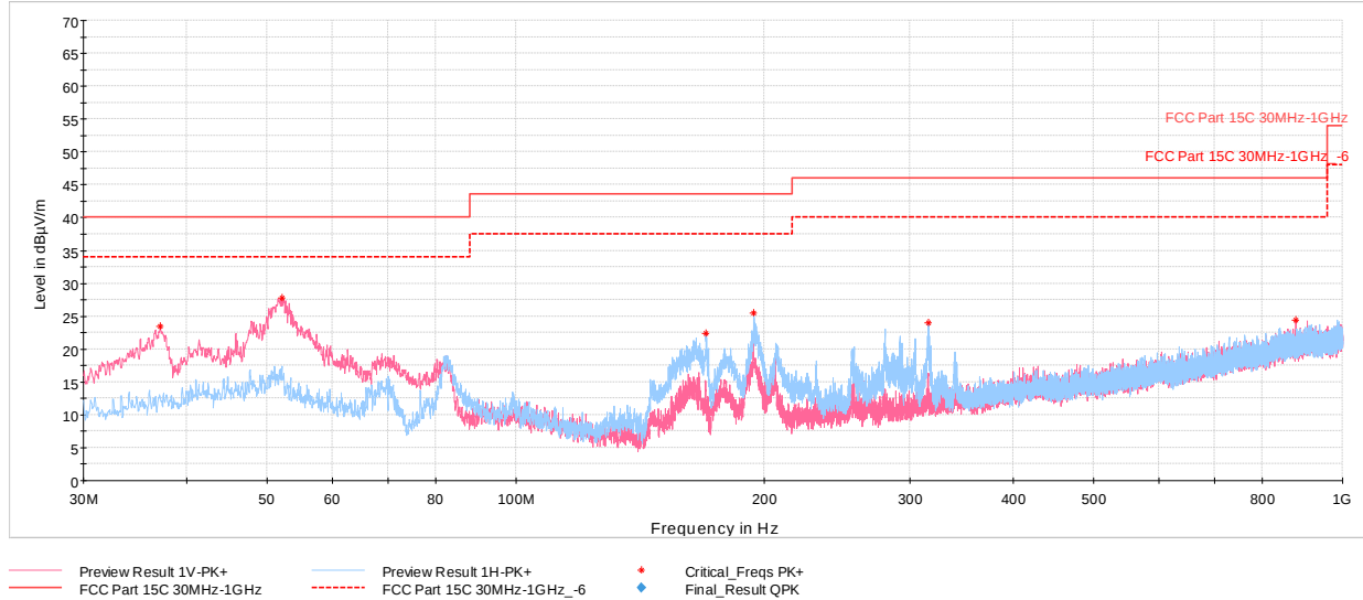
Plot 7-103. Radiated Spurious Emissions Below 1GHz TxBF (4Mbps, ePA – Ch.38 with AC/DC Adapter)
