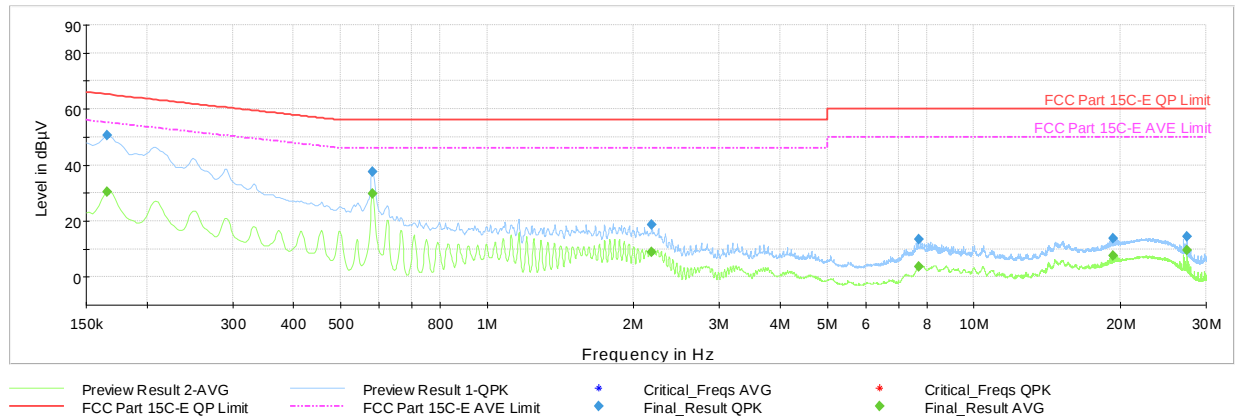
Plot 7-104. AC Line Conducted Plot with Bluetooth HDR Tx BF (L1, 4Mbps ePA - Ch.38 with Laptop)
