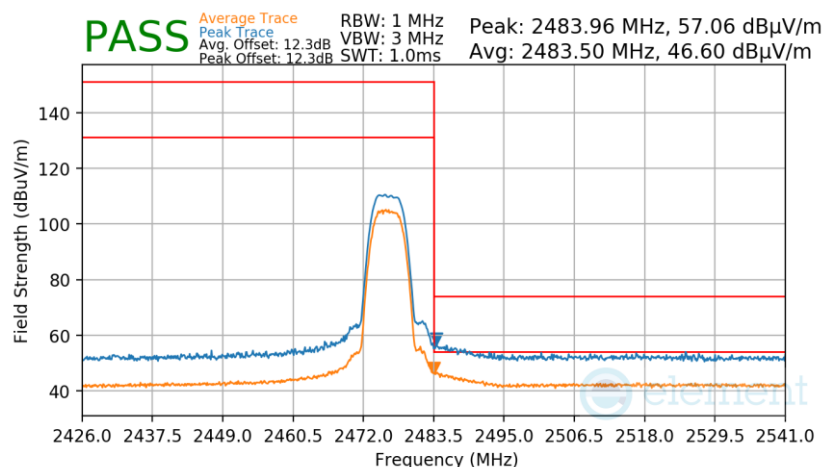
Plot 7-98. Radiated Restricted Upper Band Edge Measurement Antenna 1a
