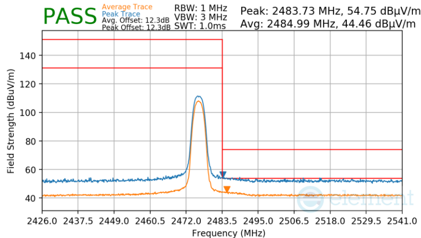
Plot 7-97. Radiated Restricted Upper Band Edge Measurement Antenna 1a
