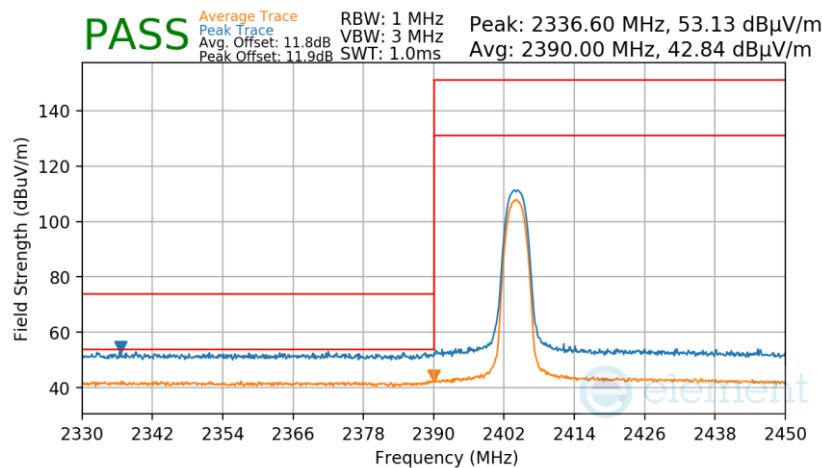
Plot 7-95. Radiated Restricted Lower Band Edge Measurement Antenna 1a
