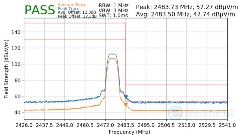
Plot 7-94. Radiated Restricted Upper Band Edge Measurement Antenna 3a
