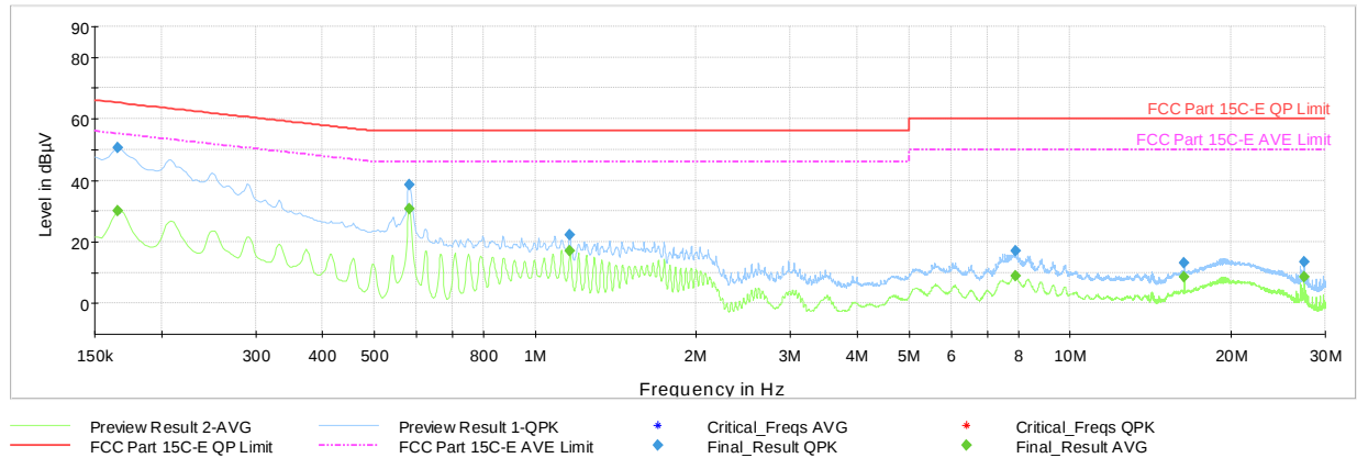
Plot 7-105. AC Line Conducted Plot with Bluetooth HDR Tx BF (N, 4Mbps ePA - Ch.38 with Laptop)
