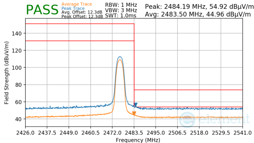
Plot 7-101. Radiated Restricted Upper Band Edge Measurement TxBF
