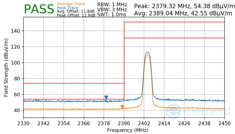
Plot 7-99. Radiated Restricted Lower Band Edge Measurement TxBF
