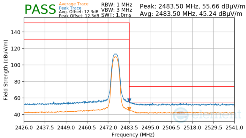
Plot 7-93. Radiated Restricted Upper Band Edge Measurement Antenna 3a
