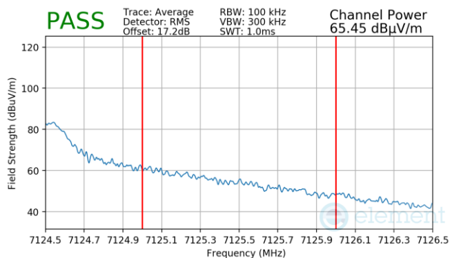
Plot 7-1534. SDM Radiated Upper Band Edge (Average – UNII Band 8)
