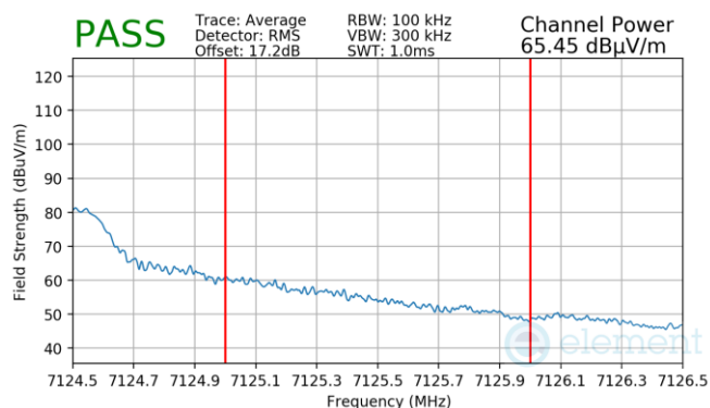
Plot 7-1504. Antenna 1b Radiated Upper Band Edge (Average – UNII Band 8)
