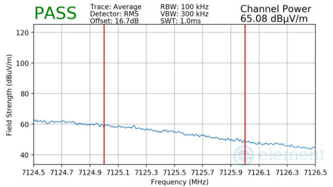
Plot 7-1488. Antenna 1b Radiated Upper Band Edge (Average – UNII Band 8)
