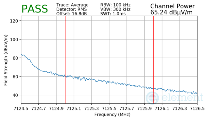
Plot 7-1530. SDM Radiated Upper Band Edge (Average – UNII Band 8)
