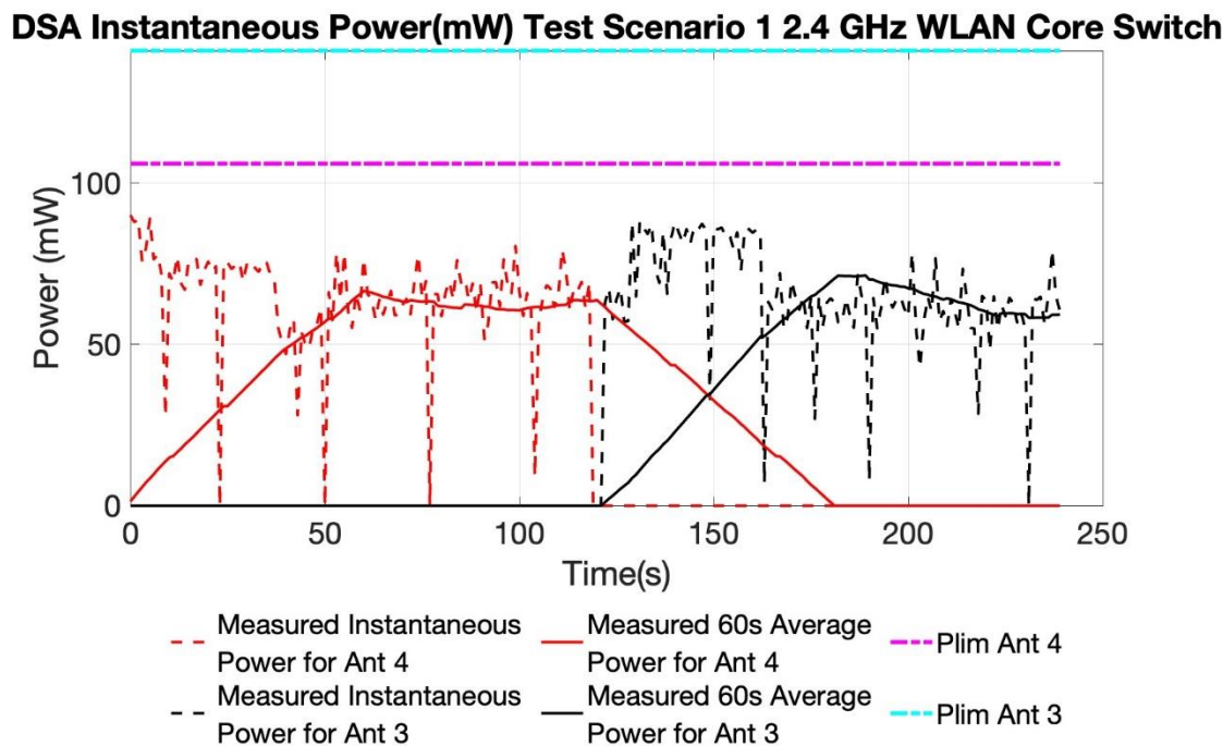
Figure 2: 60 Second Average Power vs Time, 2.4GHz
