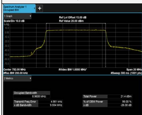
64QAM CH 23230 (782MHz)
