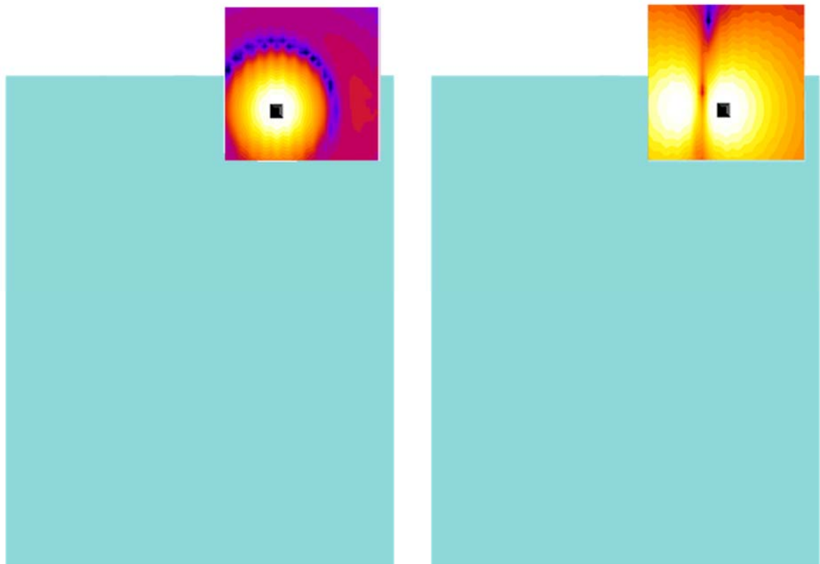
Figure 10-3 T-Coil Scan Overlay Magnetic Field Distributions (OPEN – BACK)
