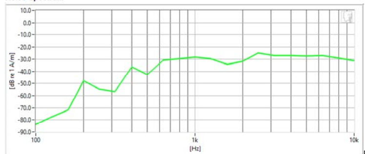
Frequency Response
