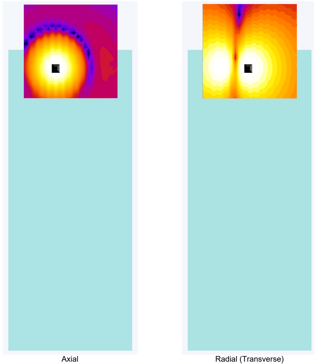
Figure 10-1 T-Coil Scan Overlay Magnetic Field Distributions
