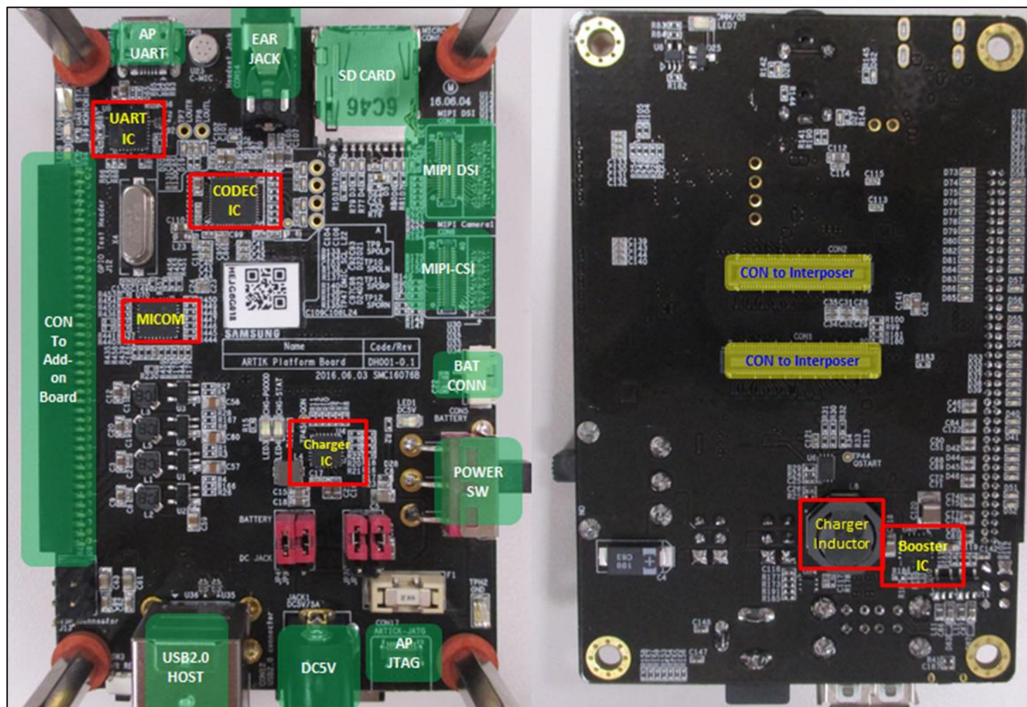
Figure 12. ARTIK 530 Development Board Platform Board Left Bottom Side, Right Top Side
