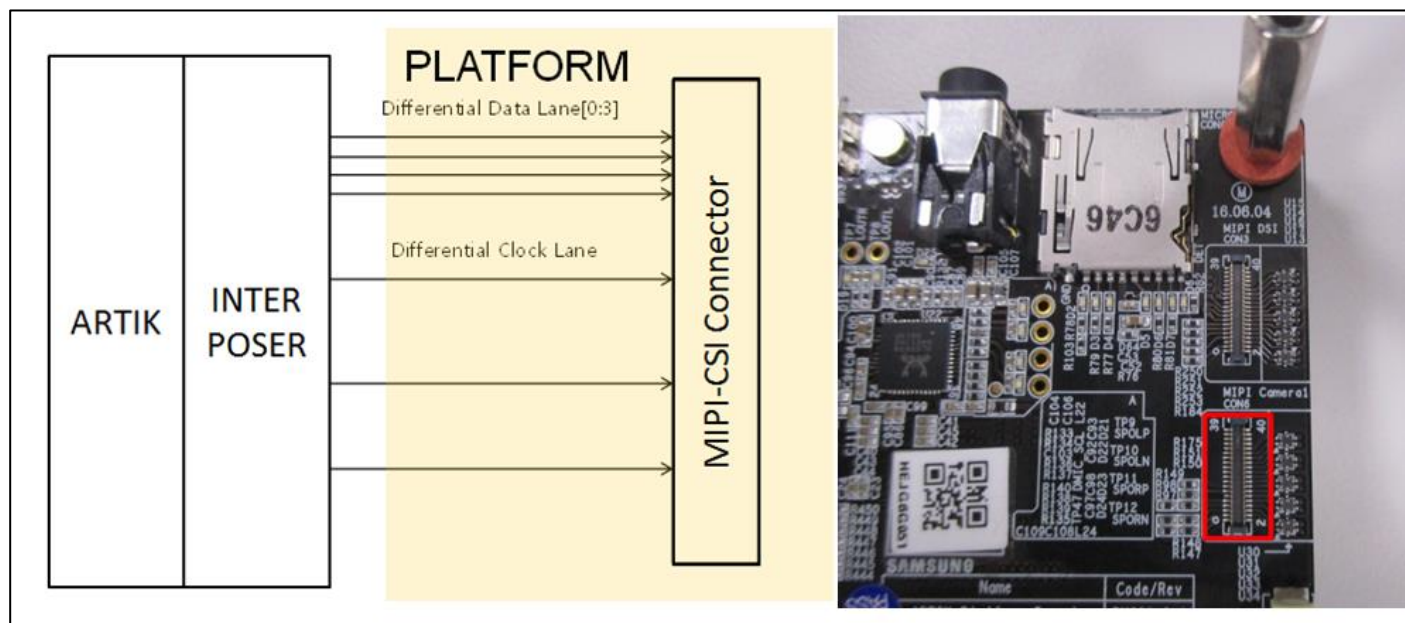
Figure 17. MIPI CSI Interface Location on the Platform Board
