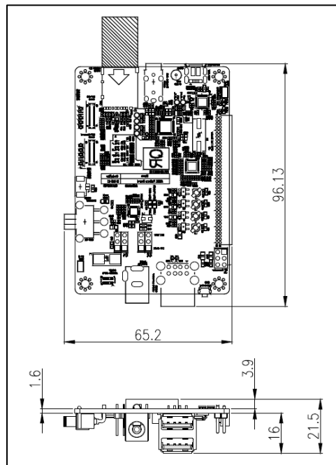
Figure 4. Mechanical Drawing ARTIK 530 Development Board Platform Board all dimensions are in [mm]
