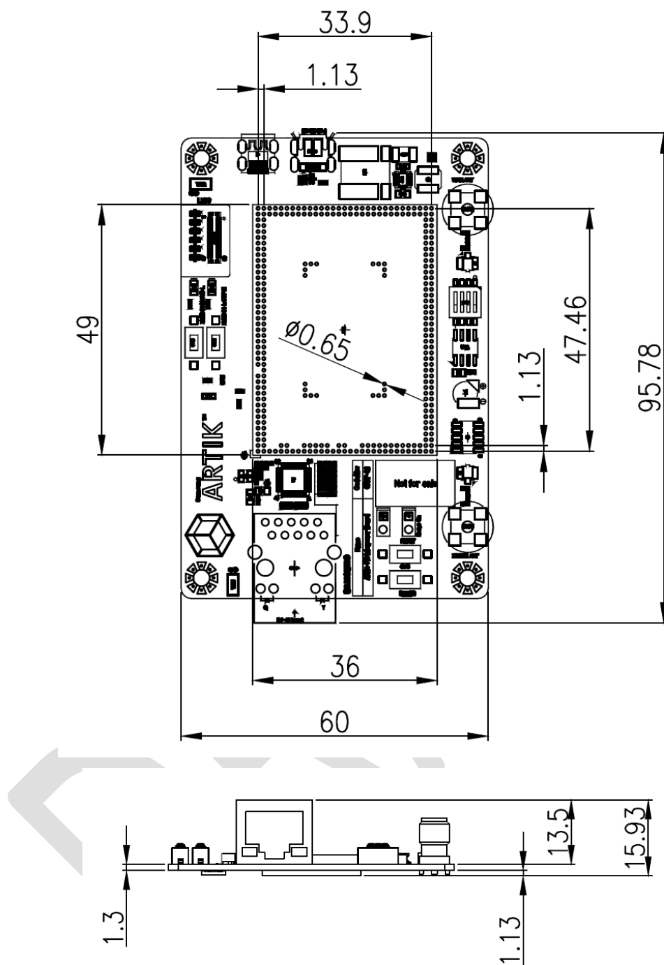
Figure 3. Mechanical Drawing ARTIK 530 Development Board Interposer Board all dimensions are in [mm]
