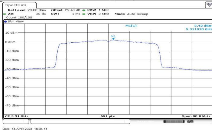
11BE40-CDD_Ant4_5310
