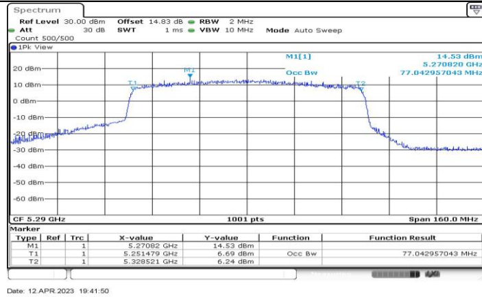
11AX80-CDD_Ant4_5290
