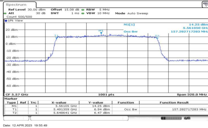
11AX160-CDD_Ant4_5570
