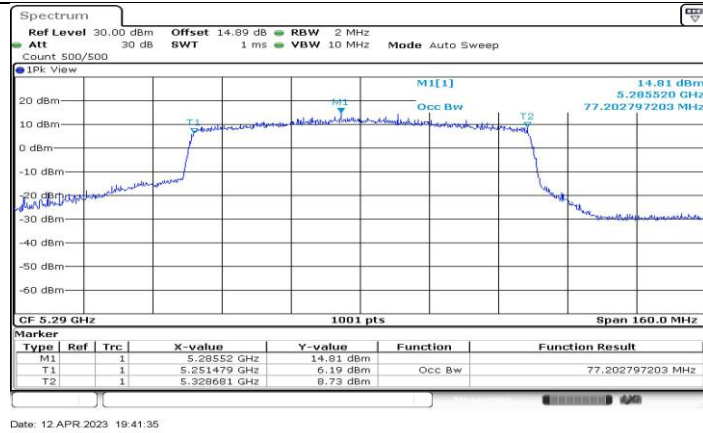
11AX80-CDD_Ant3_5290
