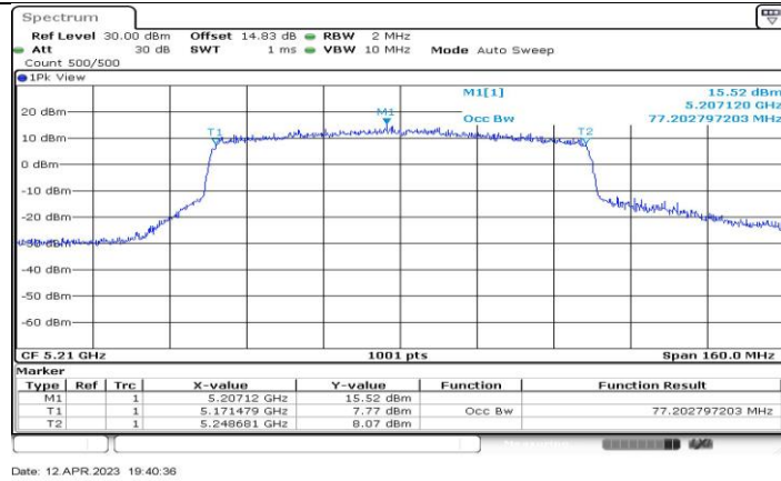
11AX80-CDD_Ant4_5210
