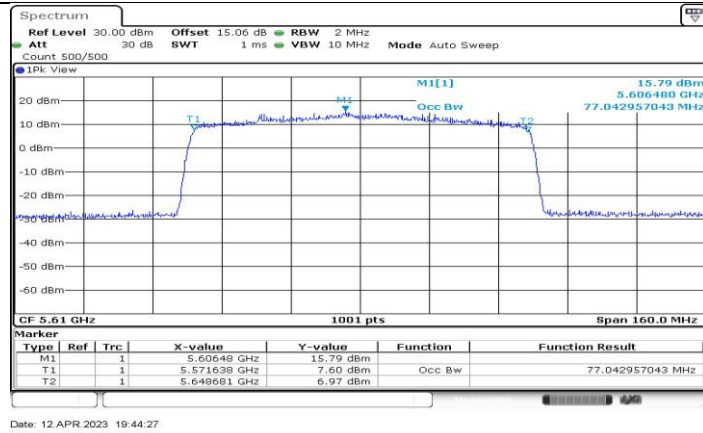
11AX80-CDD_Ant4_5610
