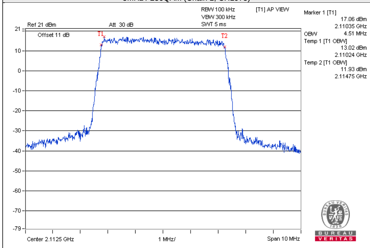
Spectrum Plot of Worst Value 5MHz / 256QAM (Chain 1, CH1975)
