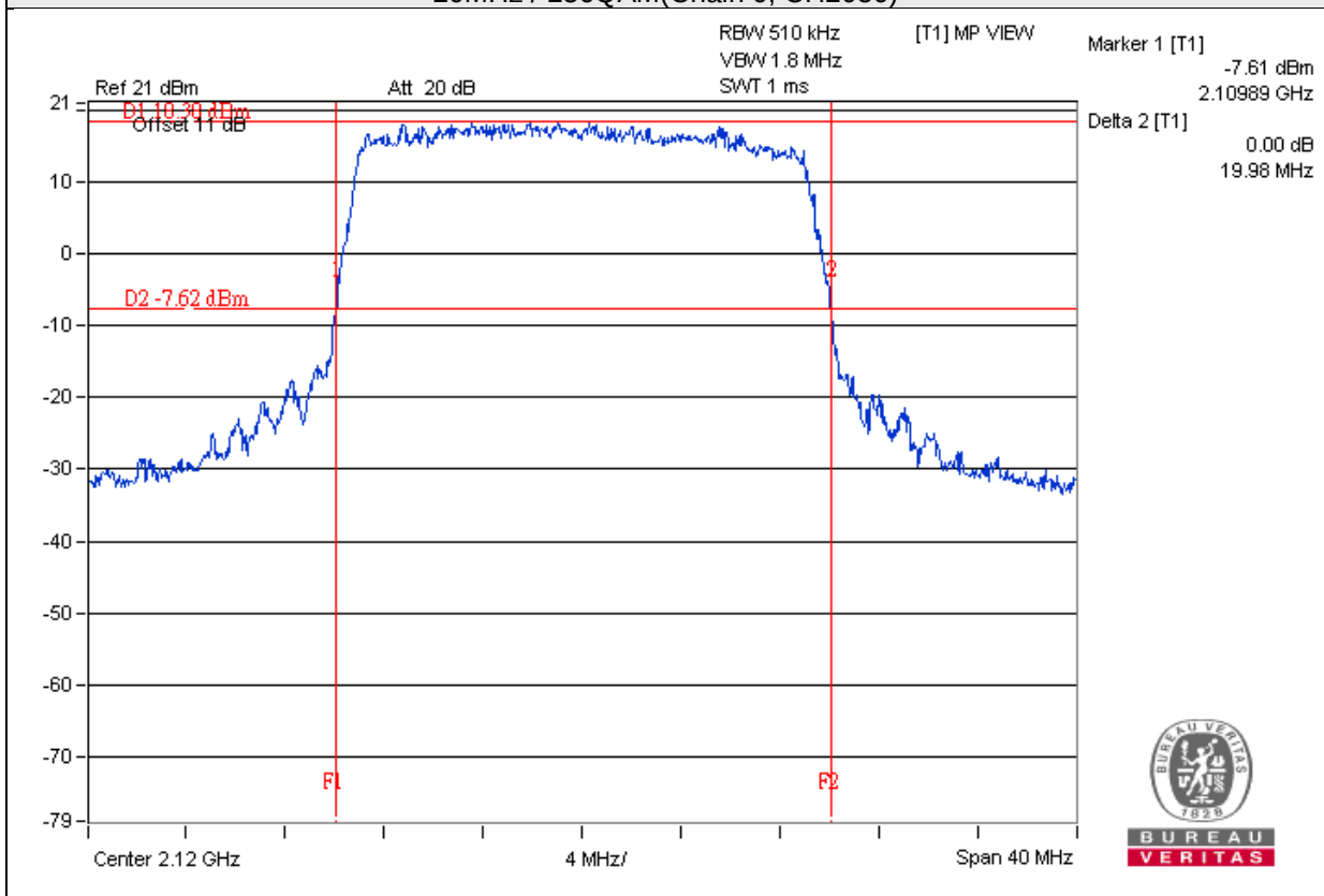
Spectrum Plot of Worst Value 20MHz / 256QAM(Chain 0, CH2050)
