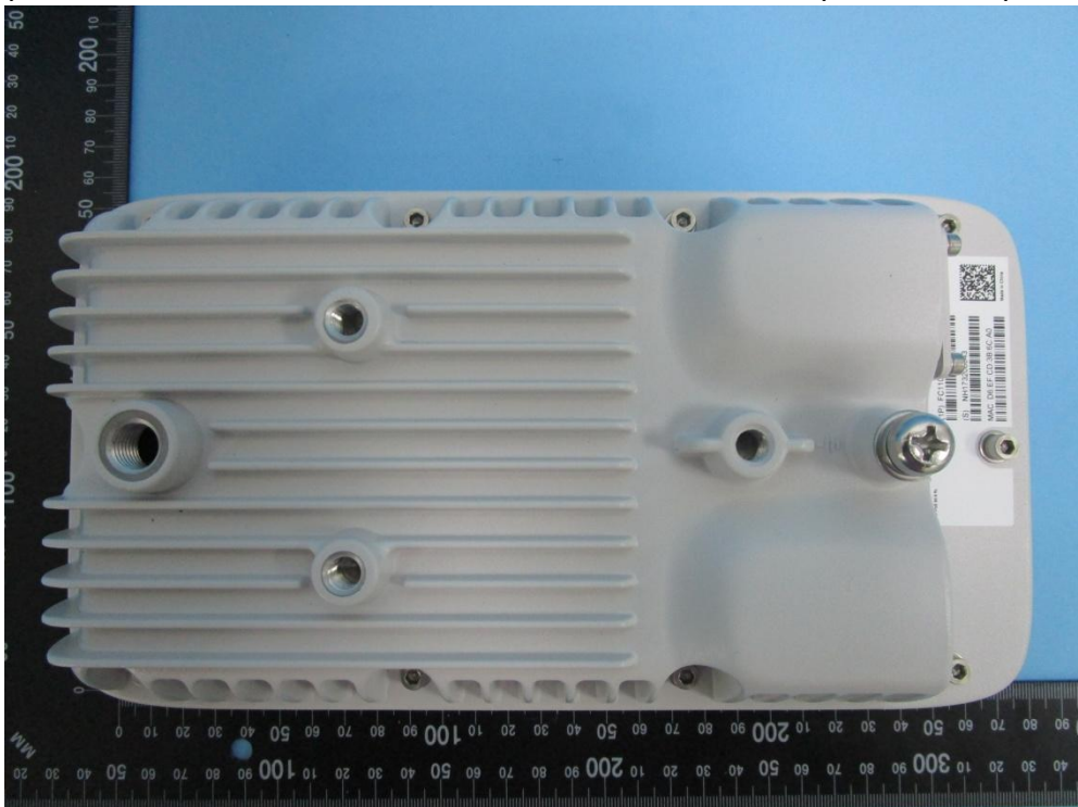
(14) External Photo - AC220 Wi-Fi AP OD omni antenna US (Bottom View)
