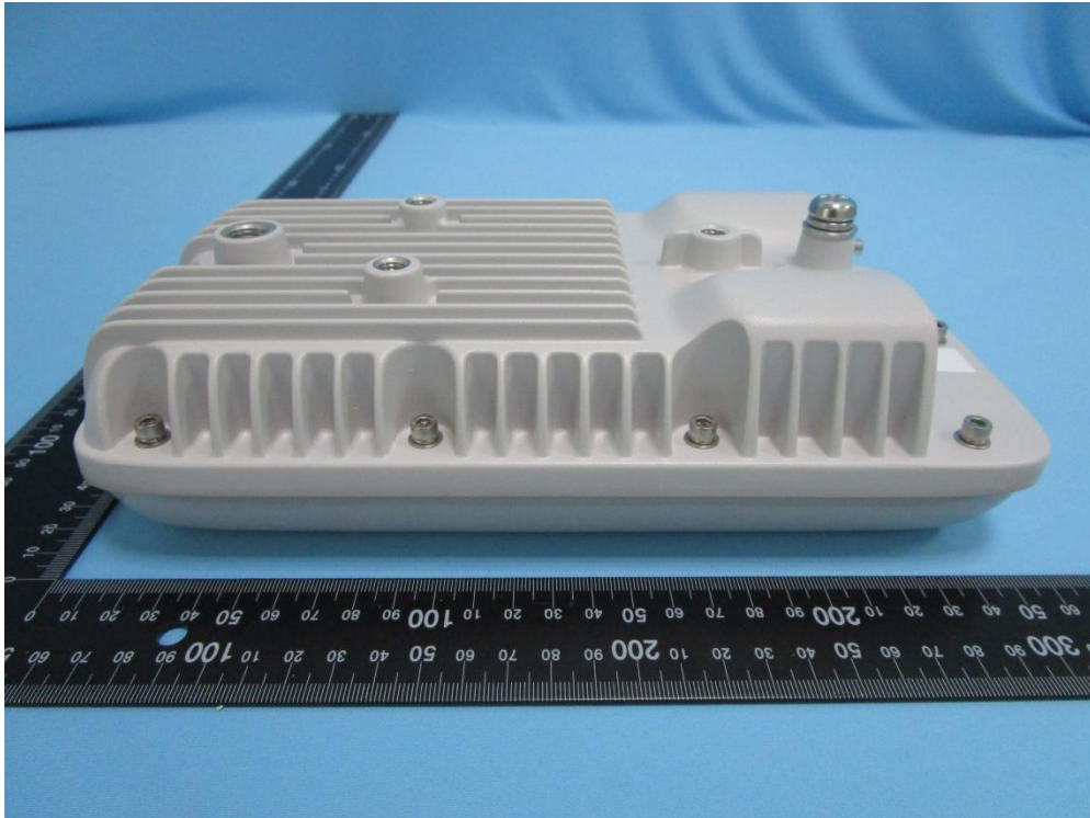
(3) External Photo - AC220 Wi-Fi AP OD directional antenna US (Side View)
