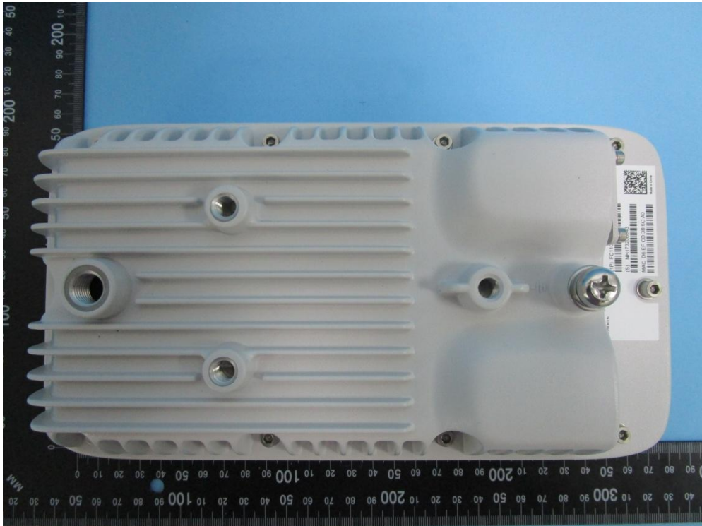
(2) External Photo - AC220 Wi-Fi AP OD directional antenna US (Bottom View)
