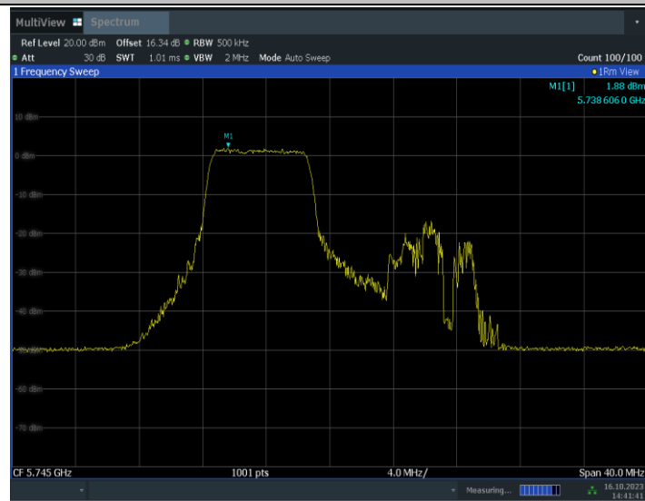
11BE20MIMO_Ant15_5745_52+26_OFDMA_1
